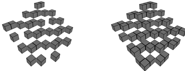
(a) A 0-connected arithmetic discrete plane ( \omega = 11 ) (b) A 1-connected arithmetic discrete plane ( \omega = 21 )
