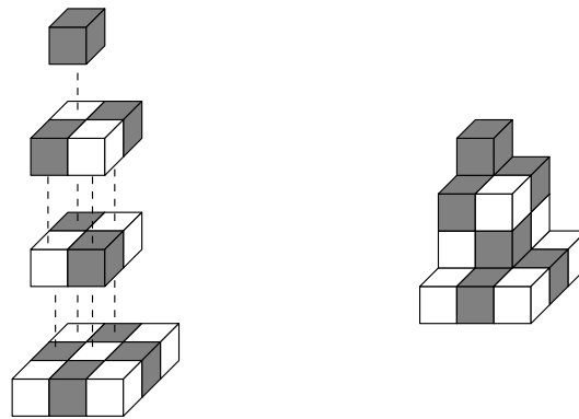
Fig. 7: Left: a sequence of bricks of a non-increasing size – Right: the associated pyramidal polycube.
