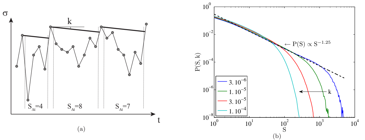
FIG. 2: (Color online) (a) Sketch of the current yield stress (as obtained in extremal dynamics) (symbol \circ ) and of the external stress when the system is coupled to a spring of constant k . Avalanches are defined as the intervals where the external stress remains larger than the yield stress. A new avalanche is initiated at the next maximum yield stress after arrest. (b) Distributions of avalanche sizes P(S, k) for a system of size L = 256 and (from right to left) different values of spring constants k = 3.10^{-6}, 1.10^{-5}, 3.10^{-5}, 1.10^{-4} . A power-law behavior P(S, k) \propto S^{-\kappa} of exponent \kappa \approx 1.25 (dashed line) is observed with a cut-off increasing as the spring constant decreases.
