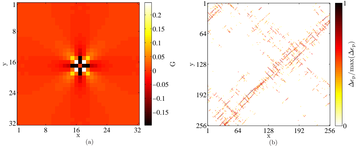
FIG. 1: (Color online) (a) Map of the quadrupolar elastic interaction G used in the model. The discretization is performed in Fourier space and an inverse Fourier transform gives in the direct space the Green function satisfying the bi-periodic boundary conditions of the problem. (b) Map of cumulated plastic activity obtained for an averaged cumulated plastic strain \Delta\varepsilon_p = 0.01 taken at \varepsilon_p = 1.0 (strain is expressed in arbitrary (infinitesimal) units). A clear localization of the plastic deformation is observed. Note that this localization behavior is non-persistent (see Ref. [16] for details on the competition between localization and diffusion of the plastic deformation.)
