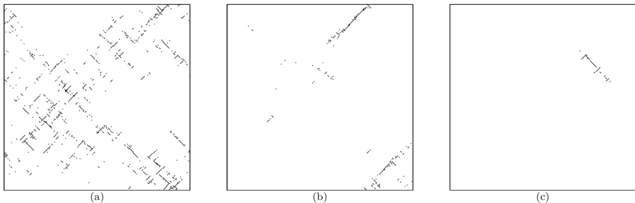
FIG. 4: Maps of cumulated plastic activity during avalanches obtained with stiffness values (from left to right) K = 10^{-1} , 10^0 and 10^1 for a system of size L = 256 . The avalanche sizes were measured to be S = 1616 , 324 and 81 respectively.
