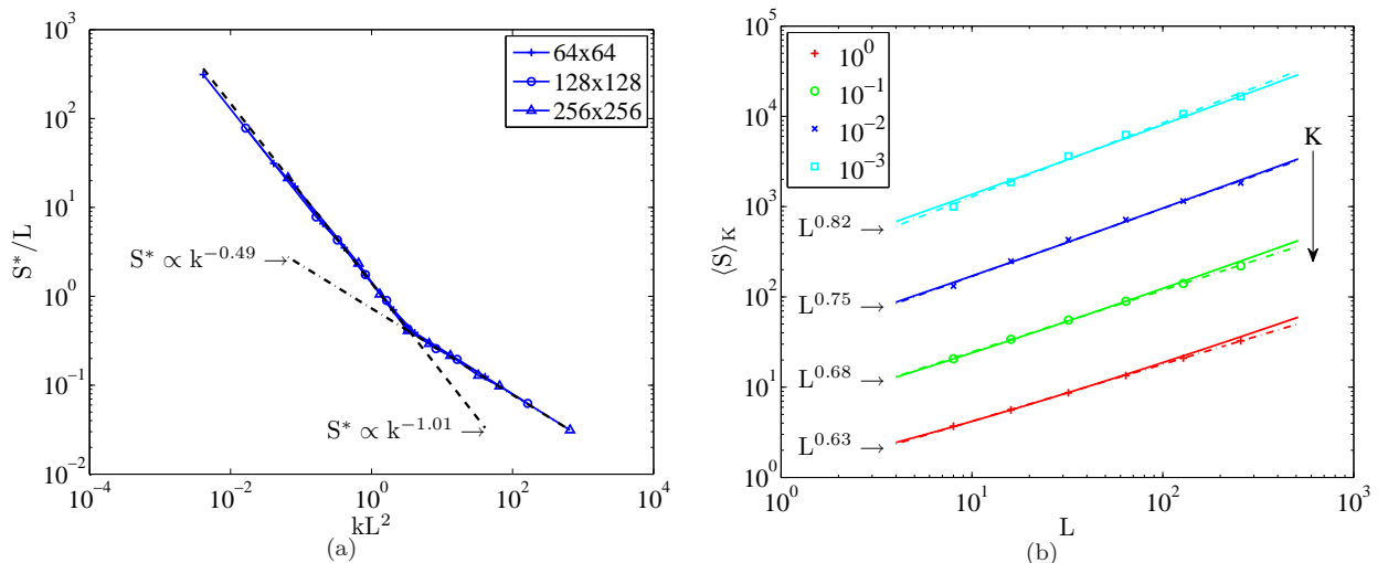
FIG. 3: (Color online) (a) Scaling of the avalanche cut-off S^* vs the rescaled stiffness K = kL^2 . The cut-off S^* scales linearly with the system size L but exhibits either an inverse or an inverse square root dependence on the stiffness K depending on K is lower or larger than the characteristic stiffness K^* = 1 . (b) Mean avalanche size \langle S \rangle_K dependence on system size L for stiffness values K = 10^{-3}, 10^{-2}, 10^{-1}, 1 . The simulation data is shown as symbols while the analytic expression Eq. 6 provides the continuous curves. The dash-dotted lines show the apparent scaling associated to these different cases. The apparent scaling exponents are very dependent on the stiffness value.
