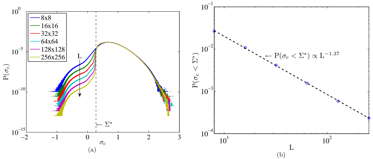
FIG. 7: (Color online) (a) Distribution of individual depinning stress P(\sigma_c(\mathbf{x})) for different system sizes L = 8, 16, 32, 64, 128 and 256 ; The dotted line indicates the macroscopic yield threshold \Sigma^* : The overcritical part ( \sigma_c < \Sigma^* ) depends on L (in contrast to the subcritical one). (b) The relative weight of the overcritical part P(\sigma_c < \Sigma^*) is observed to scale as a power-law of the system size. P(\sigma_c < \Sigma^*) \propto L^{-s} with s \approx 1.34 .
