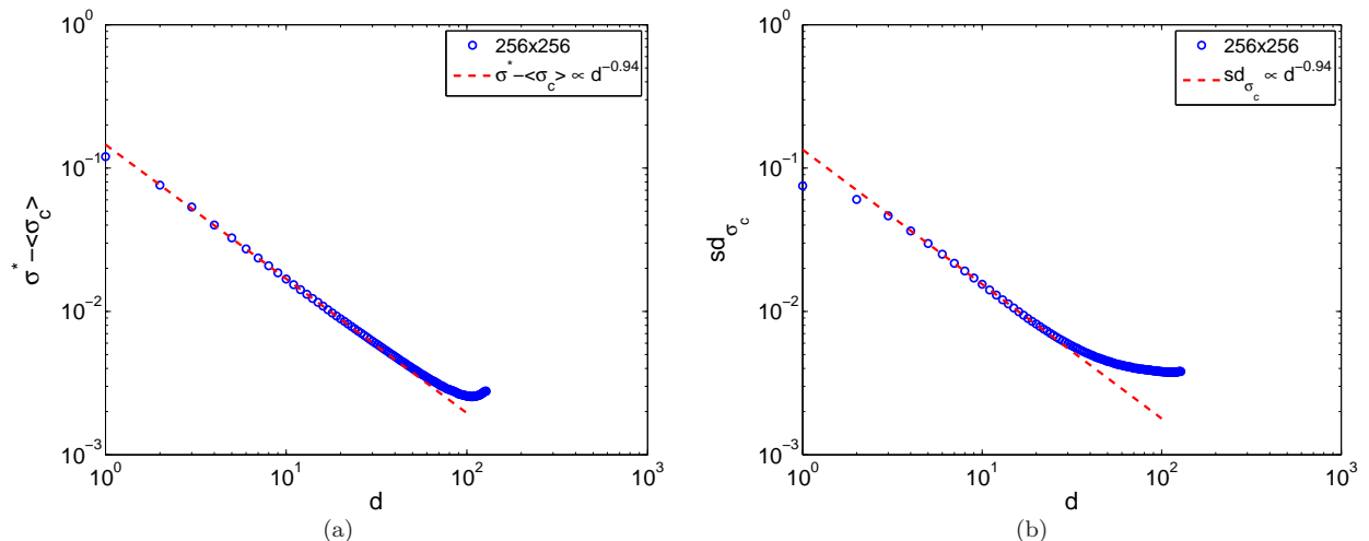
FIG. 6: (a) shows the difference between the asymptotic macroscopic yield stress, \sigma^* and the mean yield stress \langle \sigma_c(\ell) \rangle vs. distance \ell , for a system of size L = 256 . A power-law fit of exponent b \approx 0.94 is shown as a dotted line. (b) is a plot of the standard deviation of depinning stress w as a function of the distance \ell , for a system of size L = 256 . A similar power-law fit of exponent b \approx 0.94 is shown as a dotted line.
