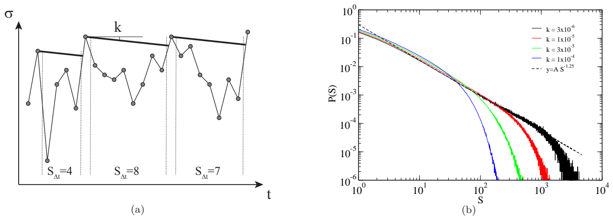
FIG. 2: (a) Sketch of the current yield stress (as obtained in extremal dynamics) (symbol \circ ) and of the external stress when the system is coupled to a spring of constant k . Avalanches are defined as the intervals where the external stress remains larger than the yield stress. A new avalanche is initiated at the next maximum yield stress after arrest. (b) Distributions of avalanche sizes P(S, k) for a system of size L = 256 and different values of spring constants k = 10^{-6}, 10^{-5}, 10^{-4}, 10^{-3}, 10^{-2} . A power-law of exponent \kappa \approx -1.25 (dashed line) is observed with a cut-off increasing as the spring constant decreases.
