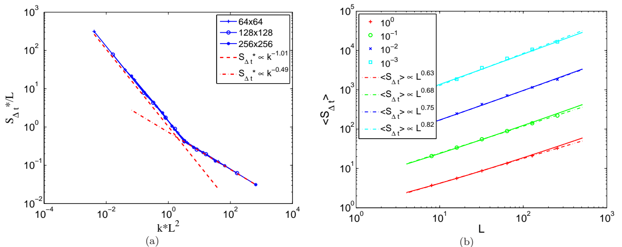
FIG. 3: (a) Scaling of the avalanche cut-off vs the rescaled stiffness K = kL^2 . The cut-off S^* scales linearly with the system size L but exhibits either an inverse or an inverse square root dependence on the stiffness K depending on K is lower or larger than the characteristic stiffness K^* = 1 . (b) Mean avalanche size dependence on system size L for stiffness values K = 10^{-3}, 10^{-2}, 10^{-1}, 1 . The simulation data is shown as symbols while the analytic expression Eq. 6 provides the continuous curves. The dash-dotted lines show the apparent scaling associated to these different cases. The apparent scaling exponents are very dependent on the stiffness value.
