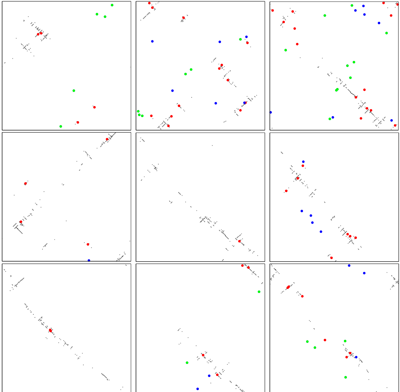
FIG. 8: Maps of cumulated plastic activity during avalanches obtained with stiffness values K = 1 for a system of size L = 256 . The colored dots indicate the location of precursors just before the avalanche takes place. Red dots are part of the avalanche, green and blue dots are not part of the avalanche but at the end of the later green dots are still overcritical while blue dots are no longer over-critical, they have been healed during the avalanche.
