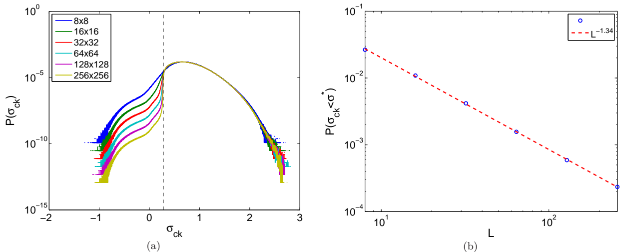
FIG. 7: (a) Distribution of individual depinning stress P(\sigma_c(\mathbf{x})) for different system sizes L = 8, 16, 32, 64, 128 and 256 ; The dotted line indicates the macroscopic yield threshold \sigma^* : The overcritical part ( \sigma_{ck} < \sigma^* ) depends on L (in contrast to the subcritical one). (b) The relative weight of the overcritical part P(\sigma_{ck} < \sigma^*) is observed to scale as a power-law of the system size. P(\sigma_{ck} < \sigma^*) \propto L^{-s} with s \approx 1.34 .
