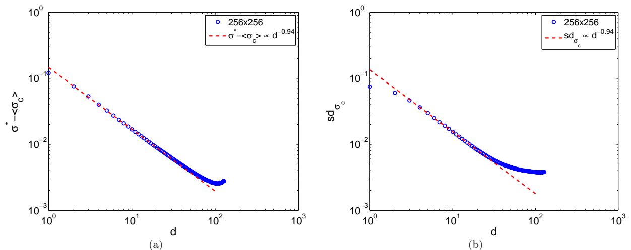
FIG. 6: (a) shows the difference between the asymptotic macroscopic yield stress, \sigma^* and the mean yield stress \langle \sigma_c(\ell) \rangle vs. distance \ell , for a system of size L = 256 . A power-law fit of exponent b \approx 0.94 is shown as a dotted line. (b) is a plot of the standard deviation of depinning stress w as a function of the distance \ell , for a system of size L = 256 . A similar power-law fit of exponent b \approx 0.94 is shown as a dotted line.
