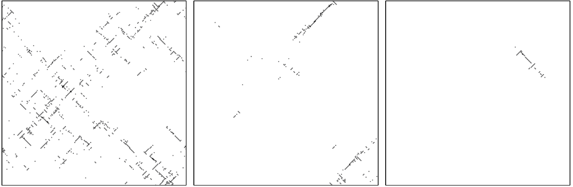
FIG. 4: Maps of cumulated plastic activity during avalanches obtained with stiffness values (from left to right) K = 10^{-1} , 10^0 and 10^1 for a system of size L = 256 . The avalanche sizes were measured to be S_{\Delta t} = 1616 , 324 and 81 respectively.
