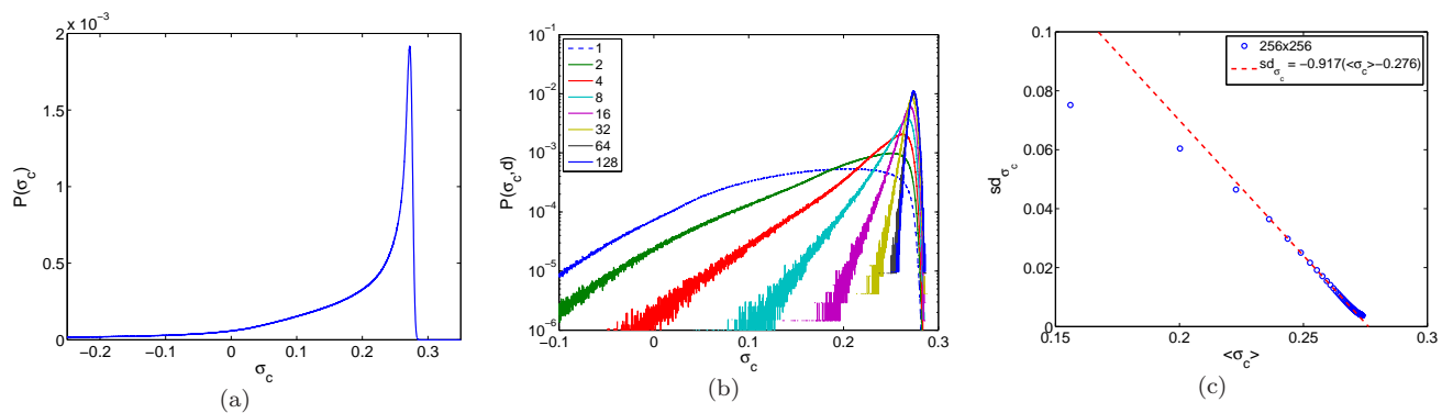
FIG. 5: (a) Distribution P(\sigma_c) of the current yield stress \sigma_c sampled over time. The macroscopic yield stress \sigma^* is given by the maximum of the distribution. (b) Representation in semi-logarithmic coordinates of the conditional distributions P(\sigma_c, \ell) such that the next slip event is located at a distance \ell from the current point. P(\sigma_c, \ell) can be interpreted as the distribution of yield stress fluctuations for a subsystem of size \ell . (c) Dependence of the width w of the distributions P(\sigma_c, \ell) vs. its mean value \langle \sigma_c \rangle_\ell for different \ell . The linear behavior obtained for large values of \ell allows to estimate the asymptotic yield limit through extrapolation to w = 0 .
