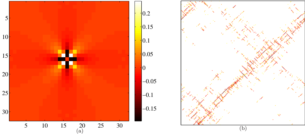
FIG. 1: (a) Map of the quadrupolar elastic interaction used in the model. The discretization is performed in Fourier space and an inverse Fourier transform gives in the direct space the Green function satisfying the bi-periodic boundary conditions of the problem. (b) Map of cumulated plastic activity obtained for a cumulated strain \Delta\varepsilon = 0.01 taken at \varepsilon = 1.0 (strain is expressed in arbitrary (infinitesimal) units). A clear localization of the plastic deformation is observed. Note that this localization behavior is non-persistent (see Ref. [16] for details on the competition between localization and diffusion of the plastic deformation.)
