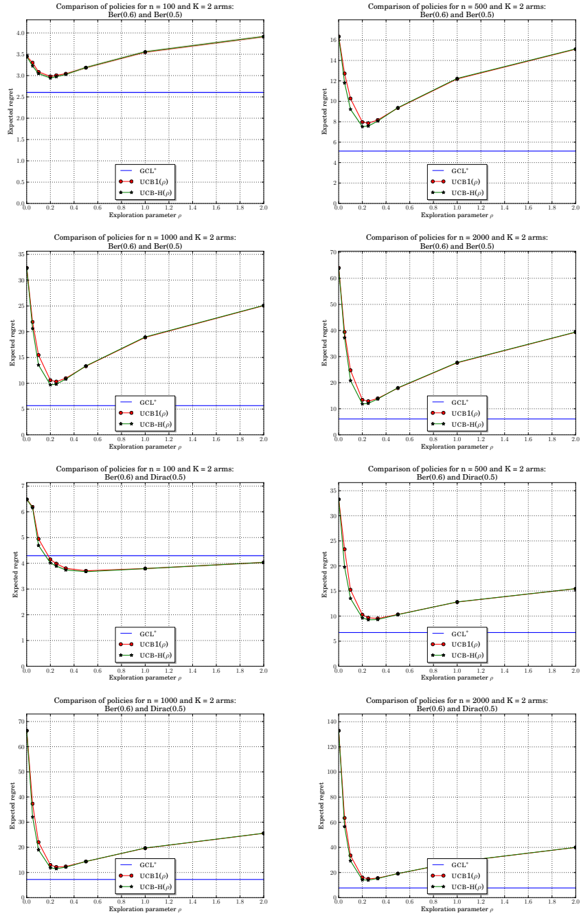
Figure 4: Expected regret of \text{UCB1}(\rho) , \text{UCB-H}(\rho) and \text{GCL}^* for various bandit settings (1/2).
