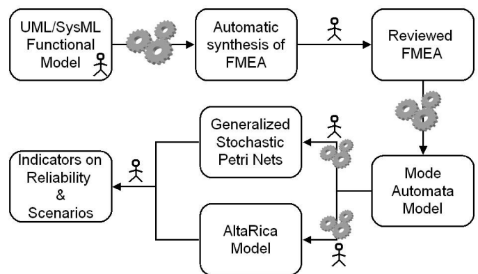
Figure 1. An approach from functional model to reliability indicators
