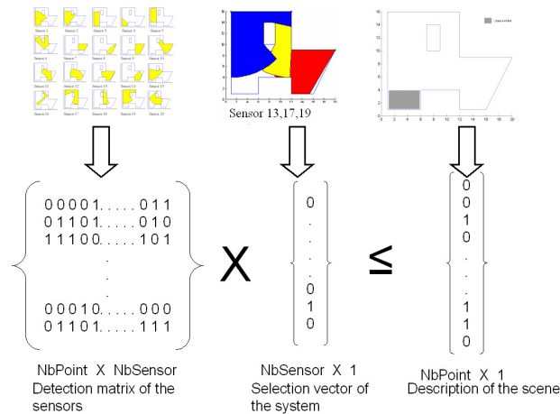
Fig. 6. Mathematical model of the placement problem
