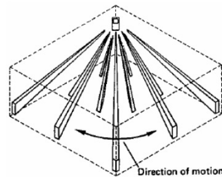
Fig. 3. Infrared rays used by an infrared movement detector (figure from [17])
