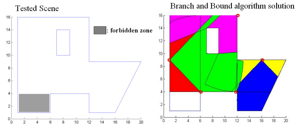
Fig. 7. Branch and Bound algorithm solution
