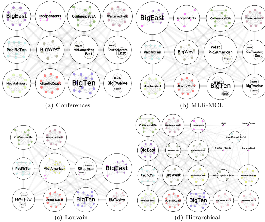
Fig. 6 Nested graph representations of the College Football conferences using several clustering algorithms.
