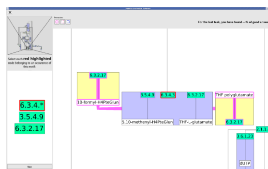
Fig. 8. Using button 2 and clicking on the reaction labelled 6.3.4.3 automatically highlights nodes at distance of at most two, and the edges and metaedges linking them. Here the reaction 6.3.4.3 is a relevant reaction since the other reactions of the motif (3.5.4.9 and 6.3.2.17) are highlighted in pink.
