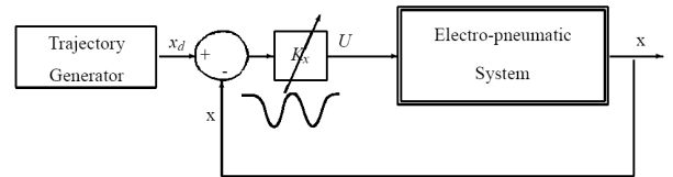
Figure 4. Position feedback control
