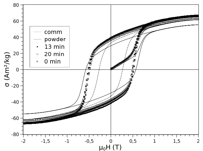
FIG. 3. Hysteresis (specic magnetization as a function of applied induction field) loops of commercial, as-calcinated and SPS sintered samples.
