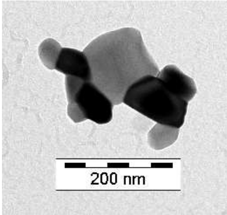
FIG. 1. Typical hexaferrite particle as received after clacination
