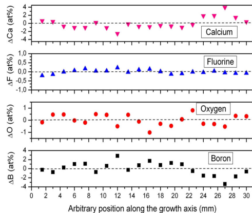
Fig. 4 – Chemical analysis of CBF fibers
