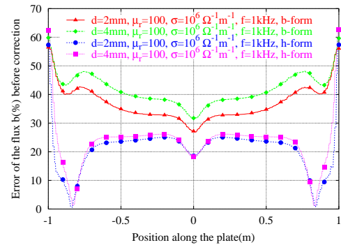
Fig. 3. Errors on the magnetic flux before correction along the plate with different thicknesses and effects of \mu_r , \sigma and frequency f
