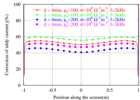
Fig. 5. Errors on the eddy current along the screen for b - formulation with effects of \mu_r , \sigma and frequency f
