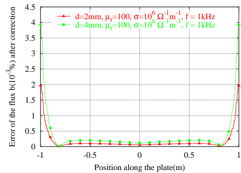
Fig. 4. Errors on the magnetic flux along the plate after correction with different thicknesses and effects of \mu_r , \sigma and frequency f
