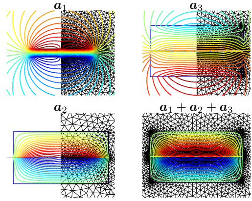
Fig. 2. Flux lines (real part) for the total solution ( a_1 + a_2 + a_3 ), the stranded inductor model ( a_1 ), thin shell added ( a_2 ) and volume solution ( a_3 ) with the different meshes used ( d = 4 \text{ mm} , f = 1 \text{ kHz} )
