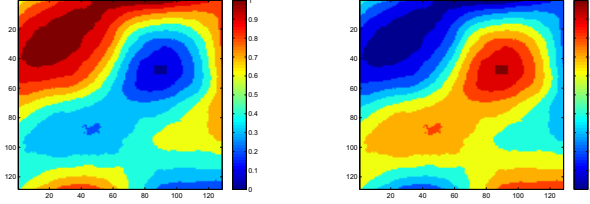
(a) Dust
