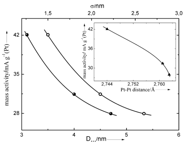
Figure 8. Mass activity of electrocatalysts at 0.72 V ( t = 200 \text{ s} ) as function of the particle size D_{111} along the <111>direction, GSD dispersion \sigma , and Pt - Pt distance.
