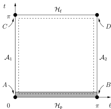
Figure 1. The Gowdy square. We assume a H^4 -regular metric and H^3 -regular time derivatives on all slices t = \text{constant} in a neighborhood (grey region) of the past Cauchy horizon ( \mathcal{H}_p : t = 0 ) and find by virtue of the results in [2], that then the metric is H^4 -regular on all future slices t = \text{constant} , 0 \leq t \leq \pi (unless the quantity J introduced in (25) is zero). In particular, a H^4 -regular future Cauchy horizon ( \mathcal{H}_f : t = \pi ) exists.
