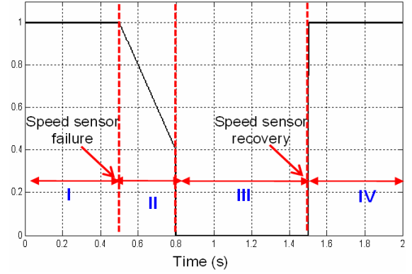
Fig. 2. Controller transition switching function ( U_s ).
