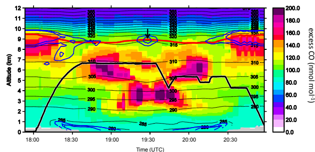
Fig. 7. FLEXPART calculations of excess CO passive tracer concentration in \text{nmol mol}^{-1} along the flight track (thick black line). The thin black lines indicate potential temperature in K, the thick red line denotes the 2 PVU isosurface, the thin blue contours show 80 and 90 % relative humidity. The arrow indicates the turning point.
