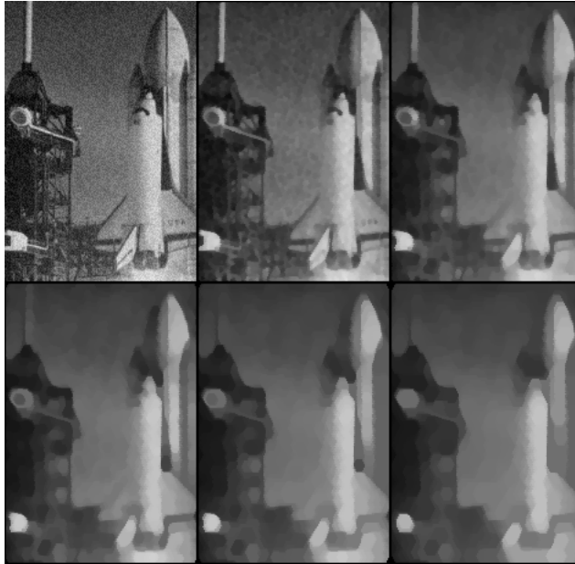
Autodial filtering. Each operator is applied on the result of the preceding one, for sizes between 1 and 5. Each operator is iterated until idempotence.
