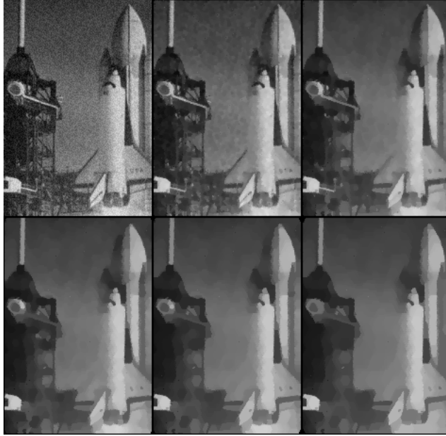
Autodial filtering. Each operator is applied on the result of the preceding one, for sizes between 1 and 5 with a constant threshold for the gradient inhibition. Each operator is iterated until idempotence
