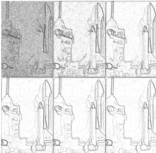
Contours of the preceding filtered image.
