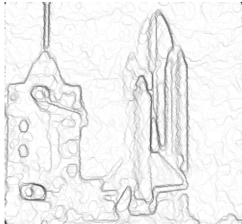
Level lines of the curvature flow (size 3, 2 iterations).
