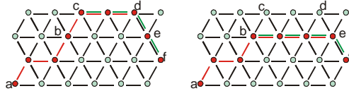
Figure 6: Left: overlapping zone of two geodesics. Right : simplification of the contour by suppression of a zone of curvature 2.
