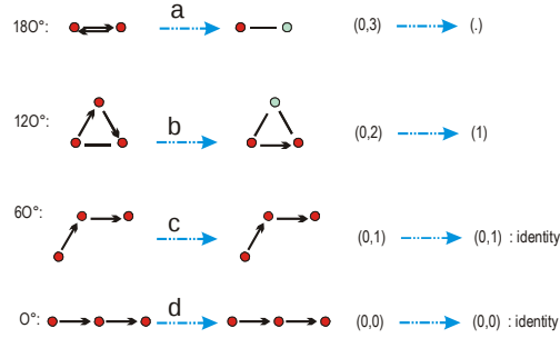
Figure 5: Inventory of the angles between two successive edges of the hexagonal raster and rewriting rules in order to simplify the contour
