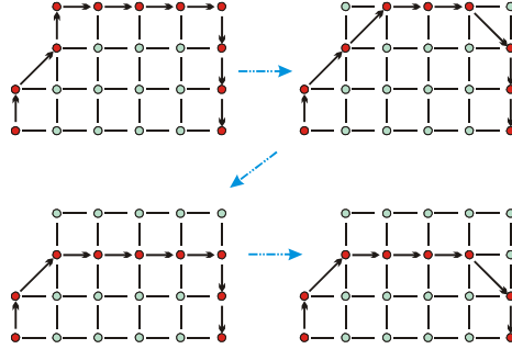
Figure 7: 3 successive simplifications of the contour in square raster and 8 connectivity
