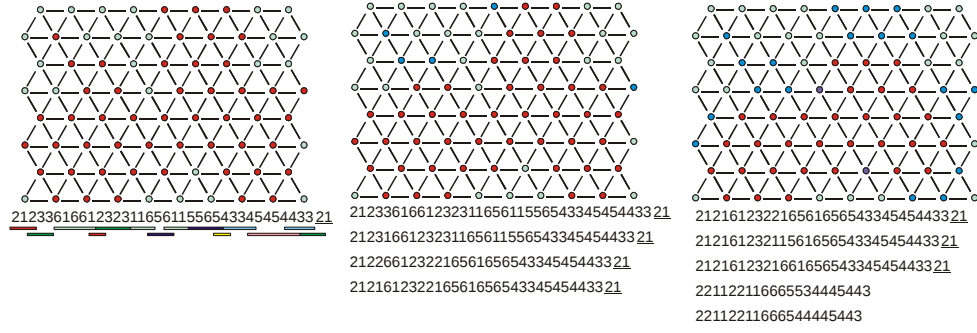
Figure 8: Left: initial image with its contour encoding. The color segments identify the geodesics. Center and right: 2 steps of curvature flow with intermediate steps of simplification of the contour encoding.
