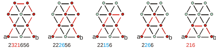
Figure 9: Suppressing zones of higher curvature may create new angular points, which are immediately and recursively suppressed until only zones of higher curvature are left.
