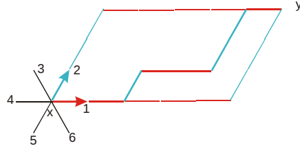
Figure 2: Geodesics between x et y , in the angular sector (\vec{1}, \vec{2}) .
