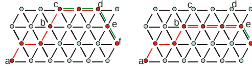
Figure 6: Left: overlapping zone of two geodesics. Right : simplification of the ontour by suppression of a zone of curvature 2.
