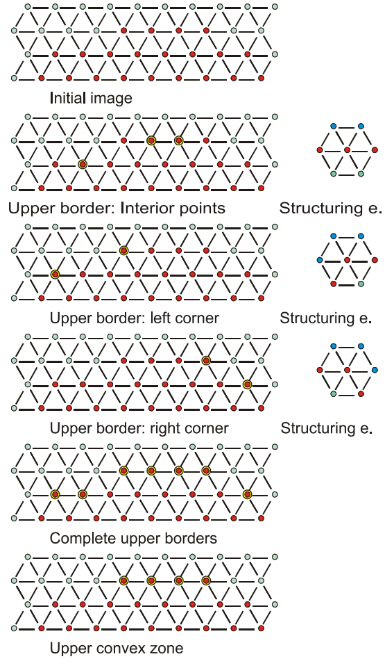
Figure 14: Algorithm for detecting an upper convex boundary based on thin- nings.
