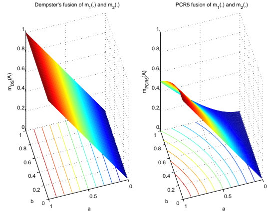
Figure 1. m_{DS}(A) and m_{PCR5}(A) for a, b \in [0, 1] .
