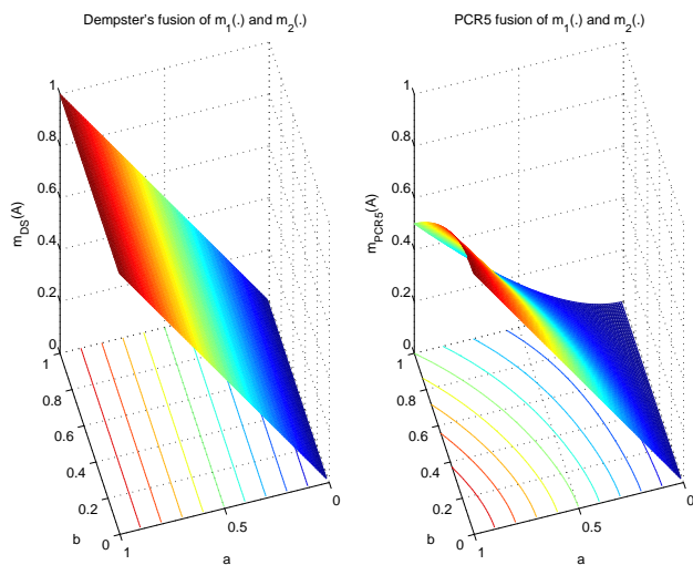
Figure 1. m_{DS}(A) and m_{PCR5}(A) for a, b \in [0, 1] .
