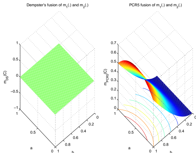
Figure 3. m_{DS}(C) and m_{PCR5}(C) for a, b \in [0, 1] .
