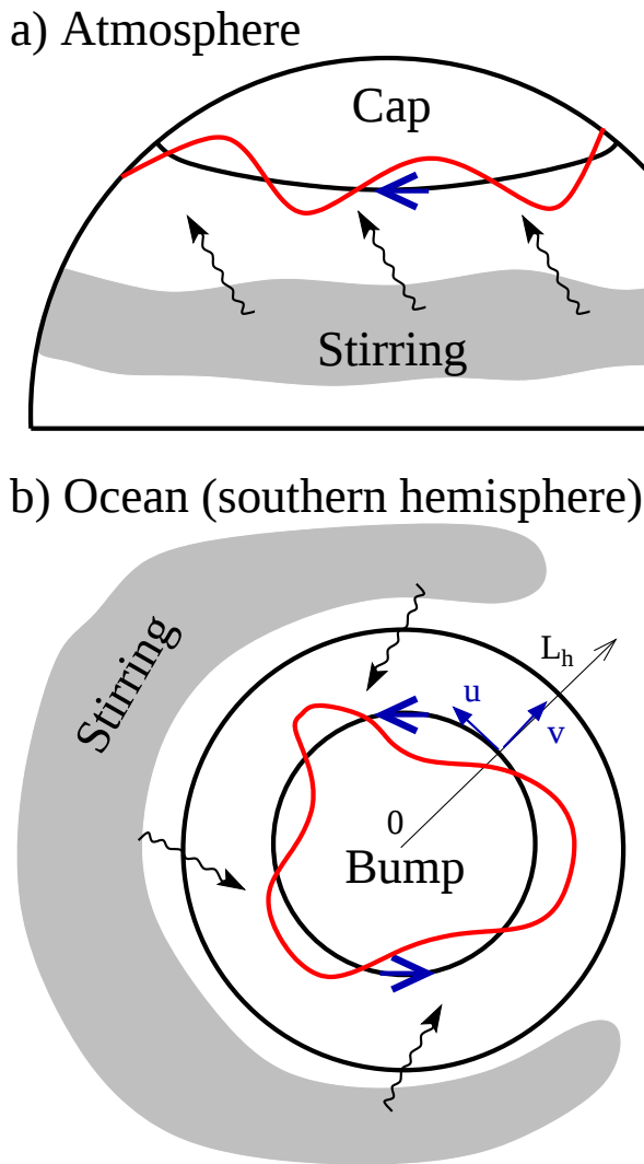
FIG. 1: Large scale flows driven by eddies in presence of a mean gradient of potential vorticity f/h . a) Case of mid-latitude atmospheric circulation: the potential vorticity gradient is due to variations of the Coriolis parameter f with latitude (beta effect). Arrows represent Rossby waves that propagate away from the stirring region and imply the formation of a westward flow outside the stirring region and an eastward flow in the stirring region [27, adapted from figures 12.2 and 12.3]. b) Case of oceanic flows above a topographic bump of typical length L_h = 600 km: the potential vorticity gradient is due to variations of depth h .
