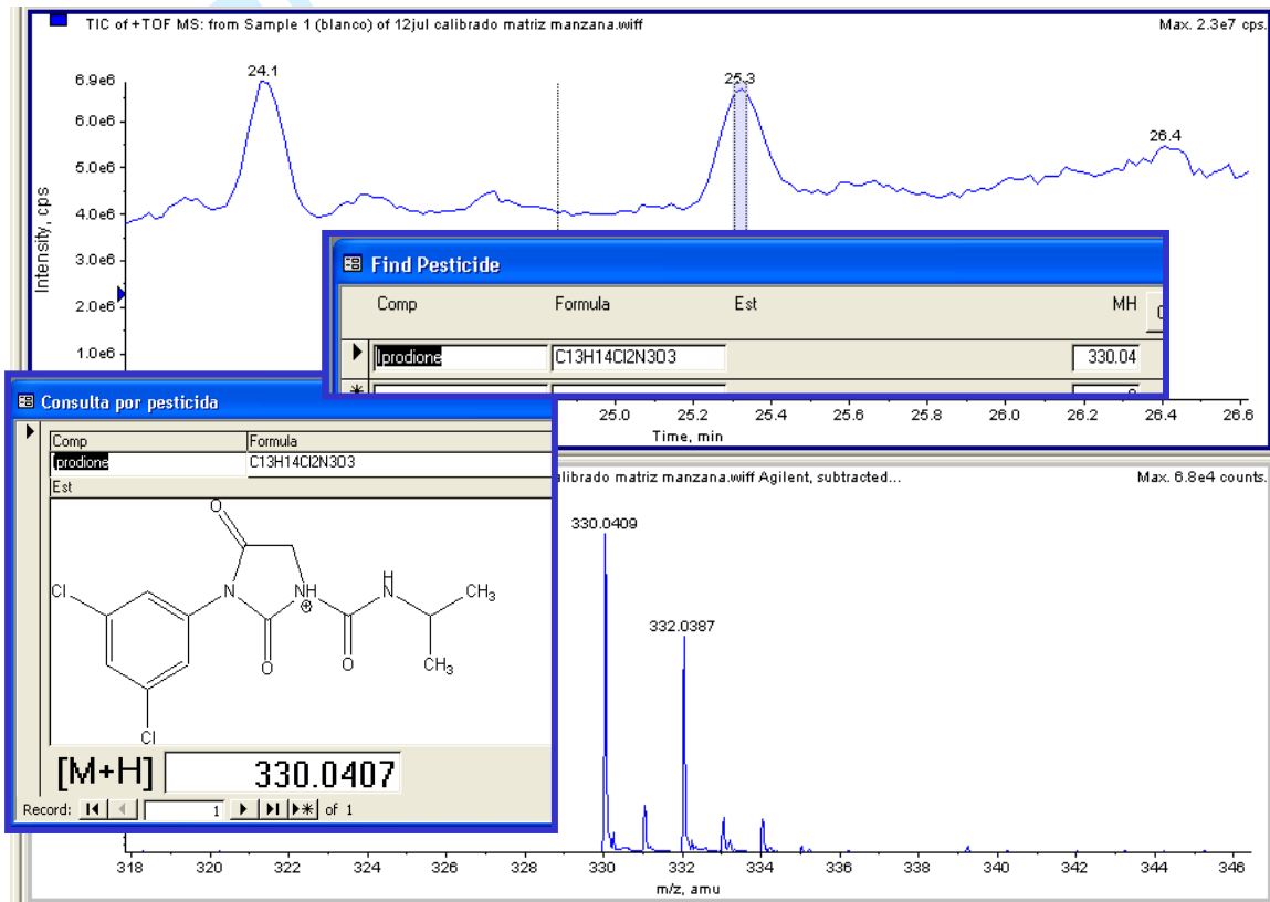
Figure 3. Accurate mass screening for mass of m/z 330.0409.
