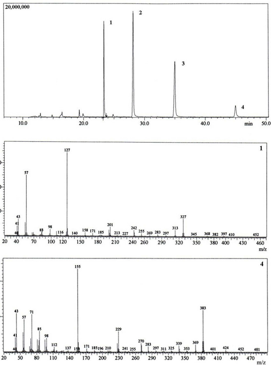
Figure 5. GC/MS trace (triglycerides group G1) produced by injection of hexane extract of organic substances (sample P84/5). Peaks are identified as follows: 1, Glycerol Tricaprylate; 2, triglycerides C26; 3, triglycerides C28; 4, Glycerol Tricaprate (sample P84/5). 180x228mm (300 x 300 DPI)
