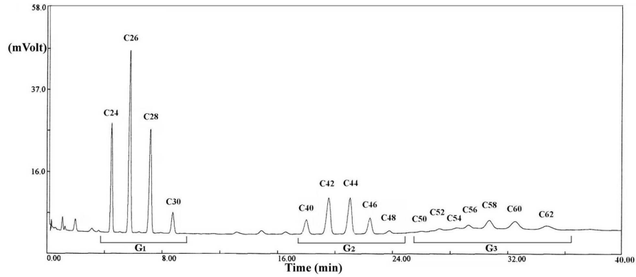
Figure 4. GC triglycerides profile, extracted from aluminium foil vessel (sample P84/3). 180x75mm (300 x 300 DPI)
