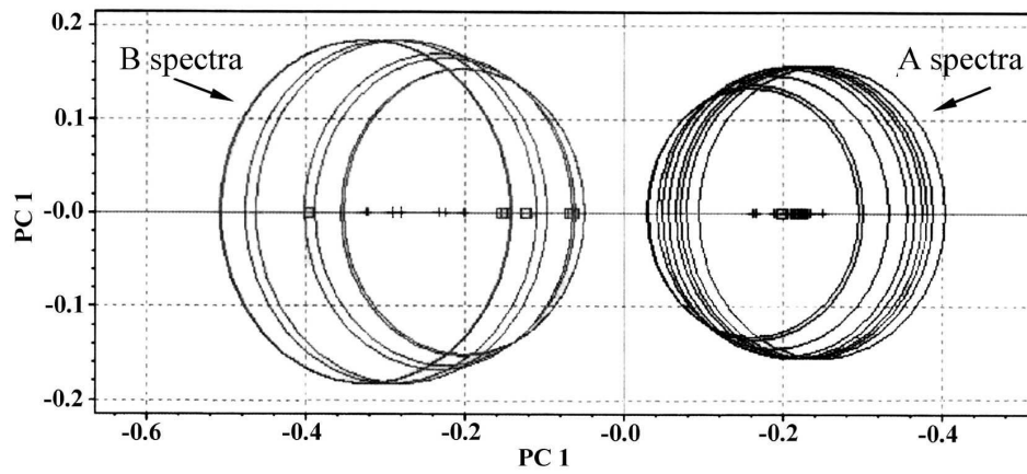
Figure 2. PCA plot, on the first principal component, for NIR spectra obtained from sample designated as P84/3. Cluster A was relevant to group A spectra (control), and cluster B to group B spectra (dishes containing extraction residue). 150x68mm (300 x 300 DPI)
