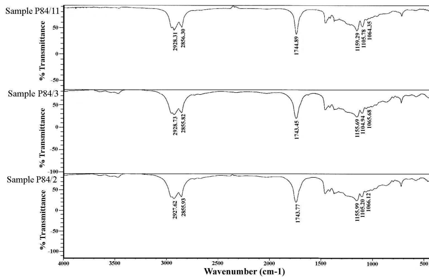
Figure 3. Comparison of FT-IR spectra of the investigated sample P84/3 together with those of samples P84/2 and P84/11. 150x90mm (300 x 300 DPI)
