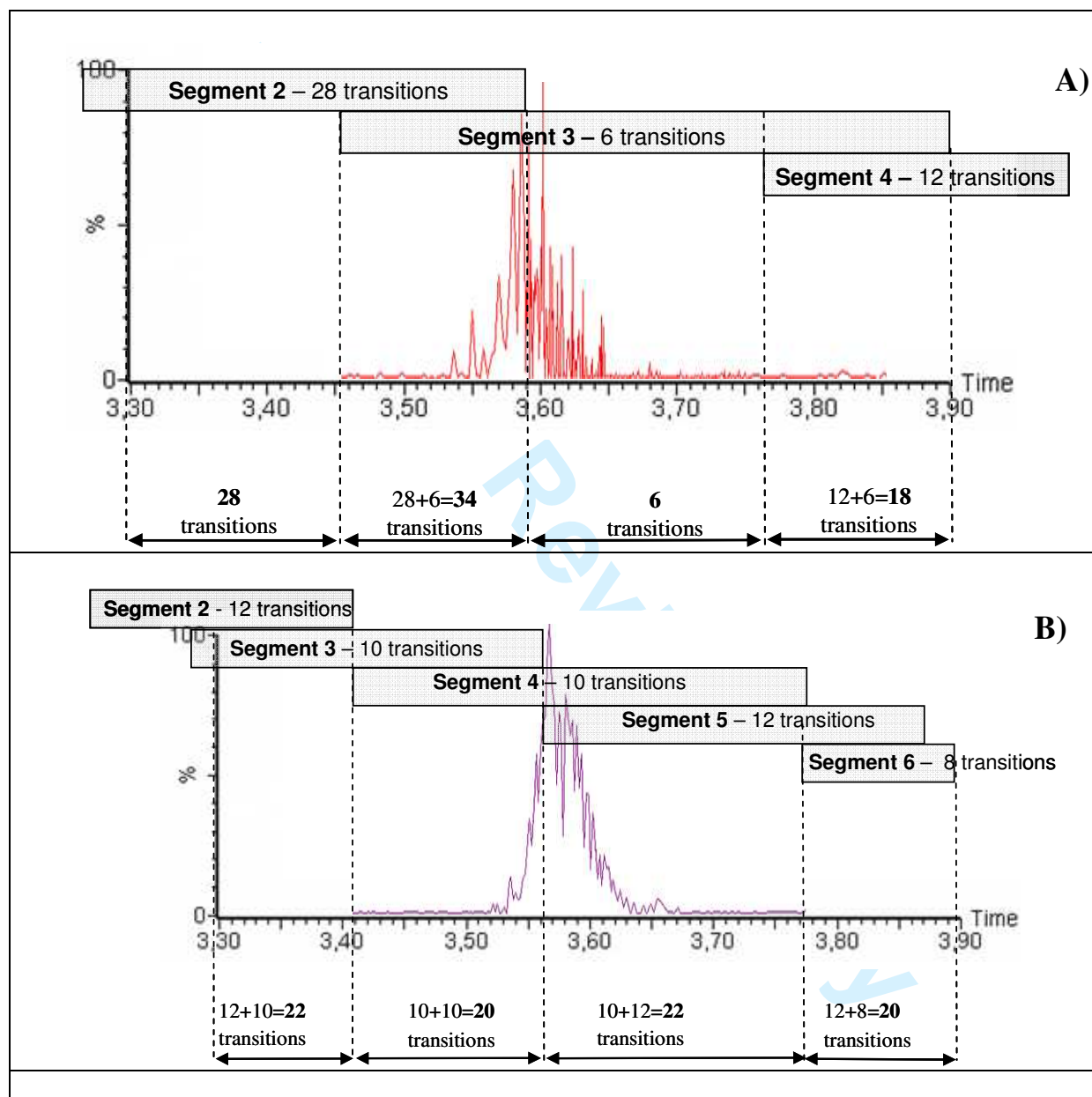
Figure 1: The impact of data acquisition setting in UPLC-MS/MS (changes of scanning frequency) on recording of analyte elution profile; aldicarb was shown as an example: In each segment a certain number of MS/MS transitions was monitored according to particular MRM method. The total number of MS/MS transitions monitored in each moment, expressed as the sum of all overlapped segments is shown below each chromatogram. The phenomenon of poor repeatability based on largely changed scanning frequencies is demonstrated on peak of aldicarb. For details see paragraph “MRM optimization”.
