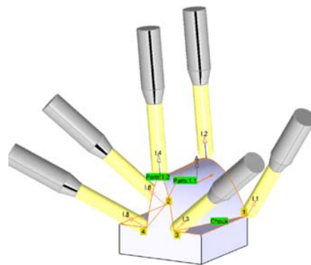
Figure 7: "interpolation" strategy
