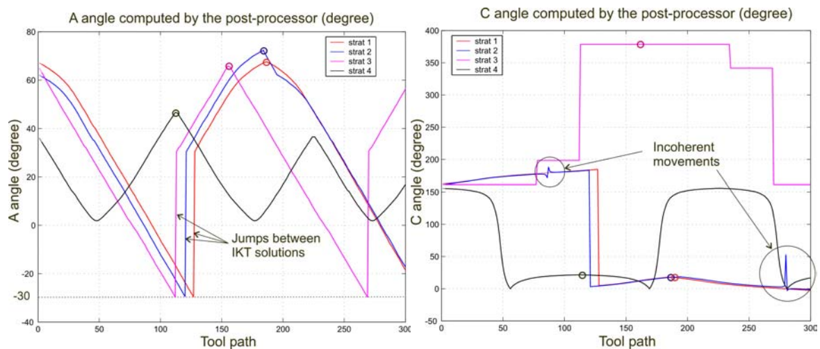
Figure 8: rotary axes commands during machining
