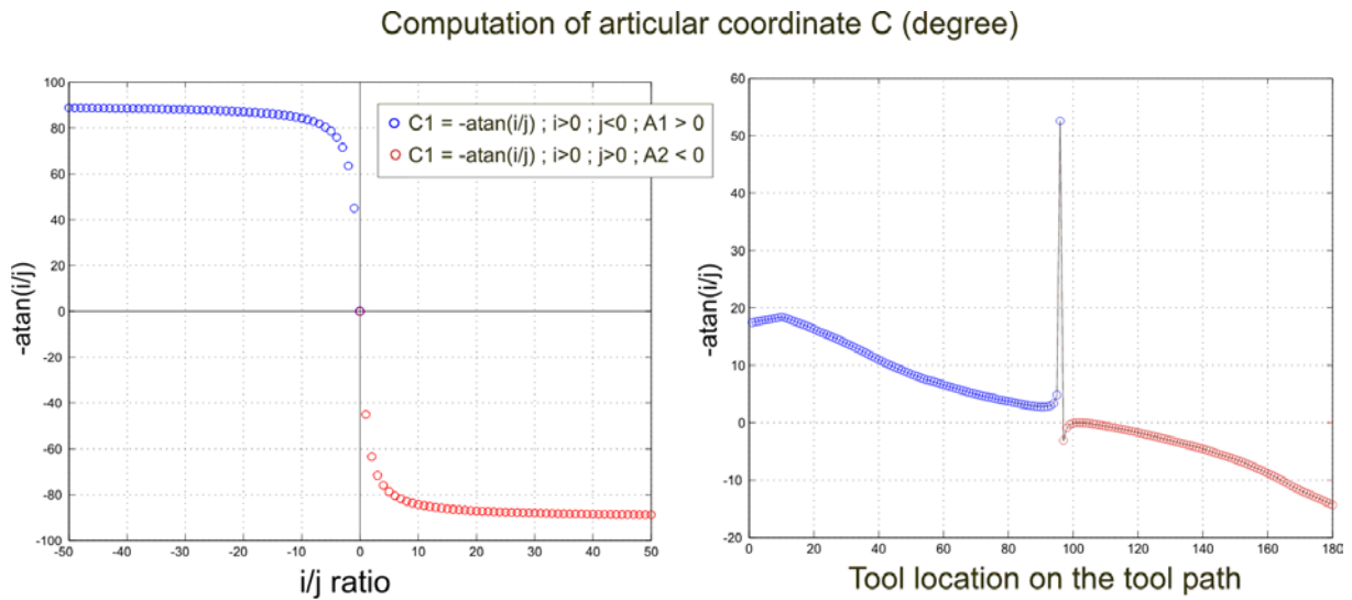
Figure 12: C axis values according to i/j ratio and to the space of solution
