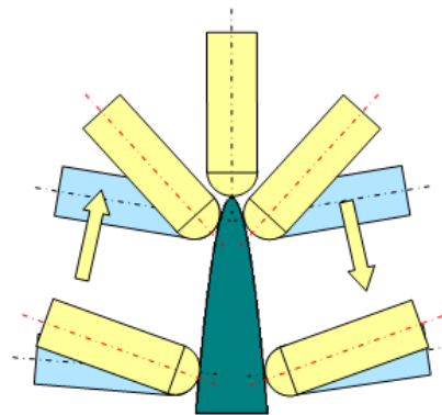
Figure 5: tool axis orientation anticipation on the leading edge.
