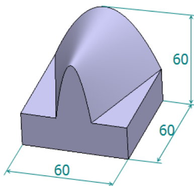
Figure 6: A axis test part
