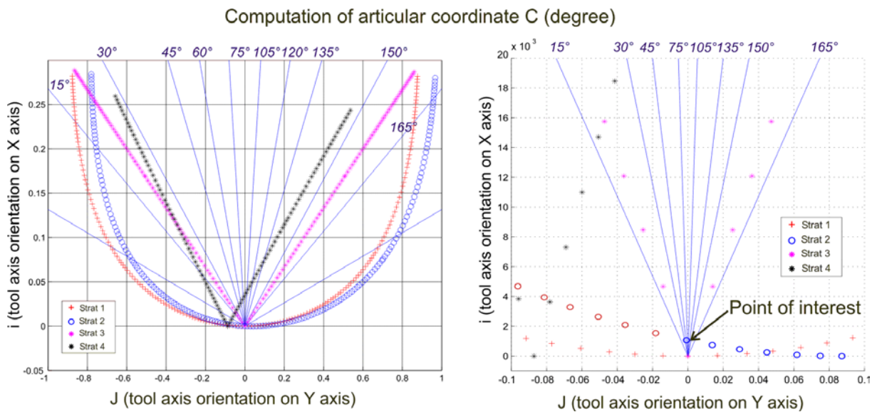
Figure 11: C axis values according to i and j
