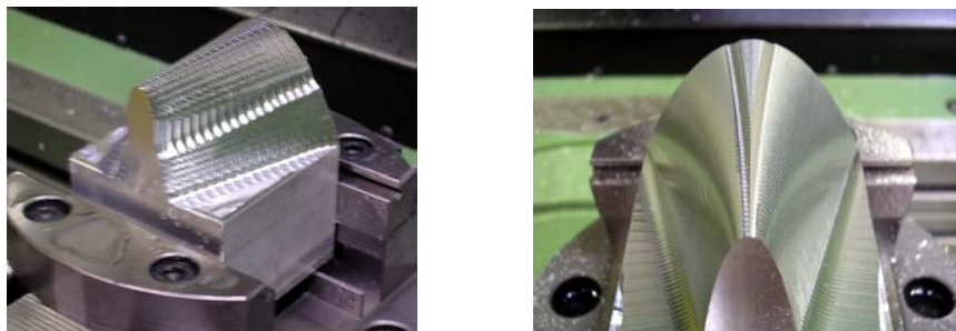
Figure 10: collisions and marks during jumps between IKT solutions
