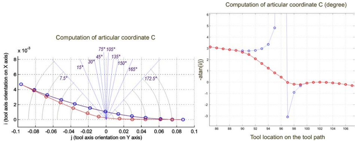
Figure 13: tool path modification in (i,j) plane
