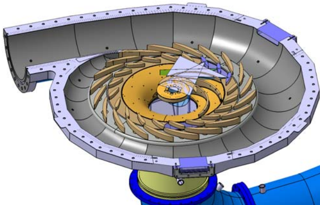
Figure 1: hydraulic pump-turbine
