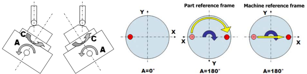
Figure 9: movement between the tool and the part according to the programming frame
