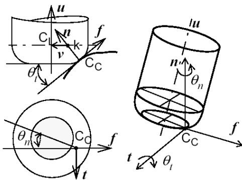
Figure 4: tool axis orientation
