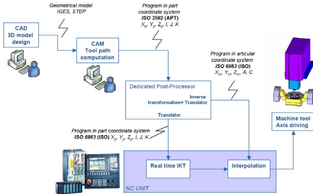
Figure 3: numerical chain in 5-axis milling
