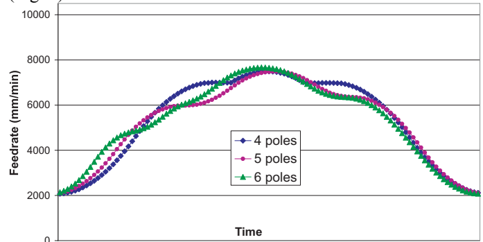
Figure 9. Feedrate evolution for each control polygon
