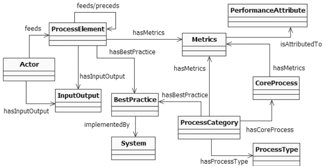
Figure 2. Entities of SCOR-KOS OWL model
