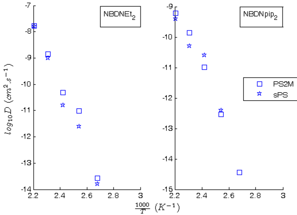
Figure 7. Comparison of the diffusion of two probes in amorphous (PS2M) or semi crystalline polystyrenes (sPS). Probes structures are given in table 2.
