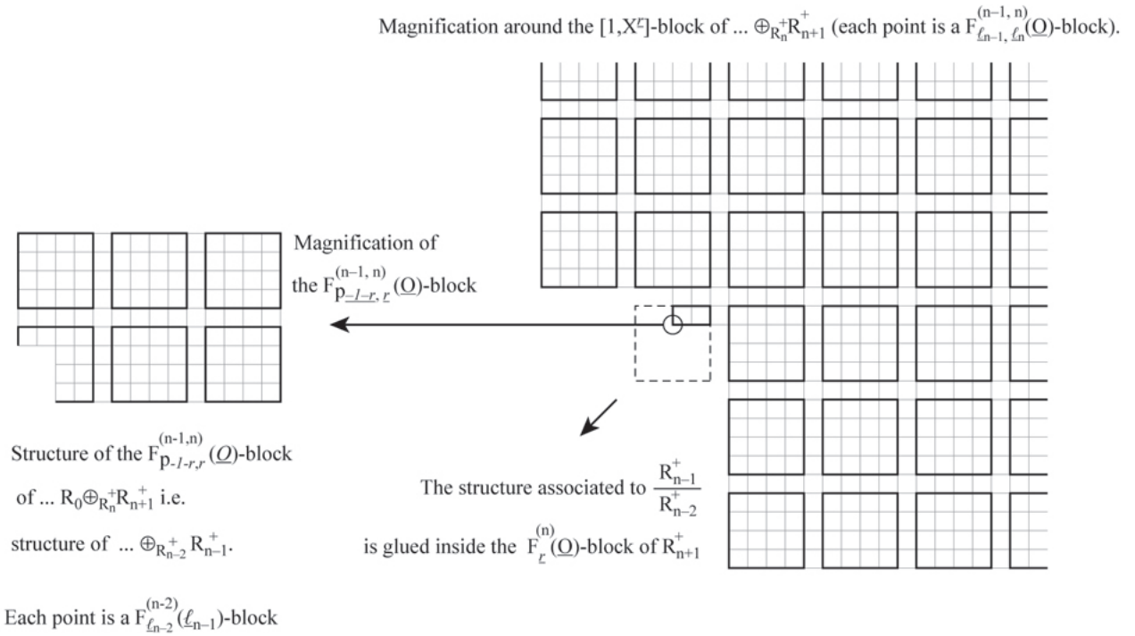
FIGURE 9: This picture shows how to glue together the datum of R_{n+1}^+/R_n^+ and R_{n-1}^+/R_{n-2}^+ (Lemma 5.13). Repeating this process for all R_{n+1-2i}^+ , i \in \mathbf{N} , i \leq \frac{n+1}{2} gives rise to a complicate fractal structure.
