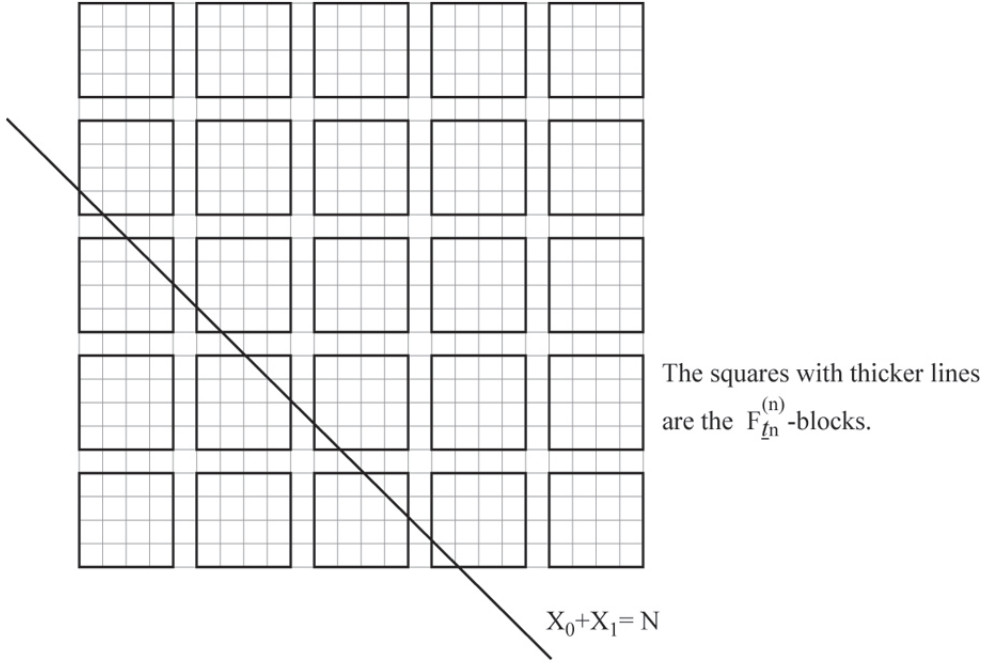
FIGURE 3: The Euclidean picture of \text{Ind}_{K_0(p^{n+1})}^{K_0(p^m)} 1 for p = 5 , m \leq n - 1 . The N -th composition factor for the socle filtration is described by the points of \mathcal{R} lying below the line X_0 + X_1 = N . Each point should be interpreted as a F_{l_{n-1}, l_n}^{(n-1, n)} -block; the square with thicker lines are then the F_{l_n}^{(n)} -blocks.
