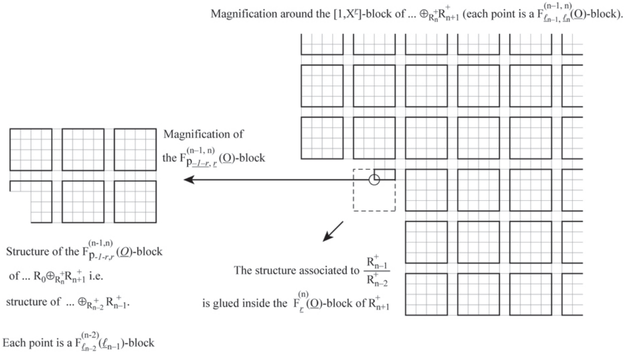
FIGURE 6: The glueing and the fractal structure in the case f = 2 , p = 5 , \underline{r} = (2, 1) . On the right side we have the particular of the [1, X^r] -block for R_{n-1}^+ \oplus_{R_n^+} R_{n+1}^+ . Notice the glueing of R_{n-1}^+ inside the F_{\underline{r}}^{(n)}(\mathbb{O}) -block of R_{n+1}^+/R_n^+ (Lemma 5.13). For the structure of R_{n+1}^+ \oplus_{R_n^+} R_{n-1}^+/R_{n-2}^+ we should further consider the F_{p-1-r, \underline{r}}^{(n-1, n)}(\mathbb{O}) -block and its magnification (left hand side). Repeating this process, we reveal the fractal nature of the structure associated to R_0^+ \oplus_{R_1^+} \dots \oplus_{R_n^+} R_{n+1}^+ .
