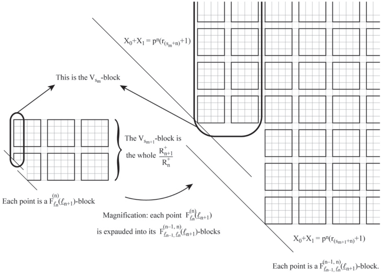
FIGURE 8: Euclidean interpretation of the filtration of R_{n+1}^+/R_n^+ by means of the subspaces (or “blocks”) \mathfrak{V}_{s_m} \subseteq \mathfrak{V}_{s_{m+1}} , in the case f = 2 , p = 5 , \underline{r} = (2, 1) . The socle of R_{n+1}^+/R_n^+ is then obtained as the sum of the points of \mathfrak{V}_{s_m} lying below X_0 + X_1 = p^n(r_{\lfloor s_m+n \rfloor} + 1) and the points of \mathfrak{V}_{s_{m+1}} lying below X_0 + X_1 = p^n(r_{\lfloor s_{m+1}+n \rfloor} + 1) (by construction, r_{\lfloor s_m+n \rfloor} \geq r_{\lfloor s_{m+1}+n \rfloor} ).
