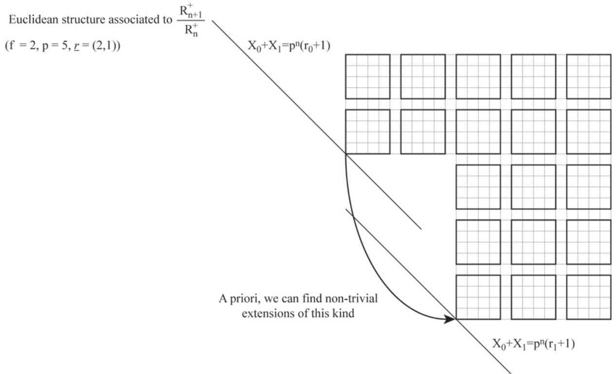
FIGURE 7: With the only Proposition 4.11 we can not exclude a priori some non trivial extensions, inside the quotient R_{n+1}^+/R_n^+ , between elements lying on hyperplanes at a distance greater than 1. In the example of the picture (again, given for f = 2, p = 5, r = (2, 1) ), we could have a non trivial extension between the elements F_{\underline{0}, \dots, \underline{0}, (3,0)}^{0,n}(\underline{0}) and F_{\underline{0}, \dots, \underline{0}, (0,2)}^{0,n}(\underline{0}) : Proposition 4.11 tells only that the subrepresentation generated by F_{\underline{0}, \dots, \underline{0}, (3,0)}^{0,n}(\underline{0}) lives in a linear space generated by a family which may contain the element F_{\underline{0}, \dots, \underline{0}, (0,2)}^{0,n}(\underline{0}) , as this element lies strictly below the hyperplane X_0 + \dots + X_{f-1} = 3p^n - 1 as soon as n > 0 .
