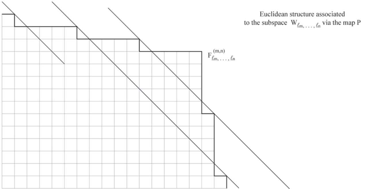
FIGURE 4: Euclidean interpretation of \mathfrak{W}_{(l_m, \dots, l_n)} for p = 5 . By Proposition 4.4 the representation generated by F_{l_m, \dots, l_n}^{(m,n)} under the action of lower unipotent matrices lives inside the linear space generated by \mathfrak{W}_{(l_m, \dots, l_n)} . Notice the fractal structure due to the behaviour of Witt polynomials.
