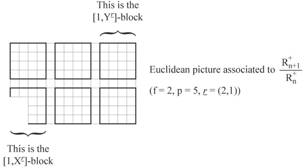
FIGURE 5: Euclidean structure for R_{n+1}^{\pm}/R_n^{\pm} in the case f = 2, p = 5, \underline{r} = (2, 1) . It is obtained as the set theoretic difference of the structures associated to R_{n+1}^{\pm} and R_n^{\pm} .
