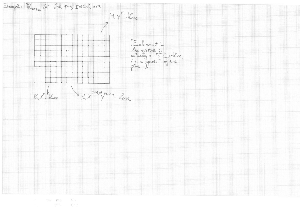
FIGURE 2: This is the structure associated to the quotient R_{n+1}^+ / R_n^+ , in the particular case p = 5 , f = 2 , r = (2, 1) . The structure of such quotients is more complicated compared to R_{n+1}^+ ; it is deduced from a delicate subdivision of R_{n+1}^+ / R_n^+ into increasing subspaces, suggested by the geometry of \mathcal{R}_{n+1/n}^+ .
