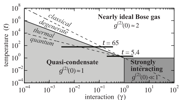
FIG. 1. Phase diagram in the interaction-temperature parameter space of a repulsive uniform 1D Bose gas [19]. The values of the local two-body correlation g^{(2)}(0) are indicated for the three main regimes (white and grey areas). The two horizontal lines show the parameters explored in this paper.
