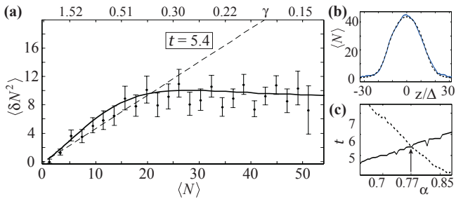
FIG. 3. (a) Variance \langle \delta N^2 \rangle close to the strongly interacting regime, for t = 5.4 . Different curves are as in Fig. 2, but for \omega_{\perp}/2\pi = 18.8 kHz, \omega_{\parallel} = 7.5 Hz, T = 40 nK ( k_B T = 0.044\hbar\omega_{\perp} ), and \kappa = 0.47 . (b) Average density profile (solid line) together with the Yang-Yang prediction (dashes). (c) The value of t obtained from fits to the density profile (dotted line) and atom number fluctuations (solid line) for different \alpha (see text).
