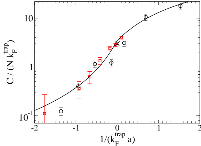
Fig. 8 The contact C = \frac{dE}{d(-1/a)} \frac{4\pi m}{\hbar^2} of a trapped unpolarized Fermi gas. The circles are obtained from the measurements of \langle N_b \rangle in [75], combined with the two channel model theory linking \langle N_b \rangle to C [Eq.(103)]. The cross was obtained in [79] by measuring the structure factor. The squares were obtained in [80] by measuring the momentum distribution. Solid line: zero-temperature theoretical prediction extracted from [29] as detailed in [69]. Here the Fermi wavevector k_F^{\text{trap}} of the trapped gas is defined by \hbar^2 (k_F^{\text{trap}})^2 / (2m) = (3N)^{1/3} \hbar \bar{\omega} , with \bar{\omega} the geometric mean of the three oscillation frequencies \omega_{\alpha} and N the total atom number.
