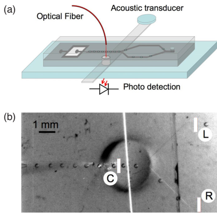
FIG. 8. (Color online) (a) Scheme of the bubble switching experiment showing the optical detection system and acoustic actuation. A 4.5\ \mu\text{m} monomode optical fiber is directly plugged into the microfluidic circuit. Light scattered from bubbles is detected on a p-i-n photodiode. (b) Top view of bubbles flowing in the microchannel with a Y junction. Bubbles are emitted from the focusing device at the left side of the picture. The bubble emission frequency is optically measured in the central C branch, their passing time in each branch is recorded at the white marks L and R.
