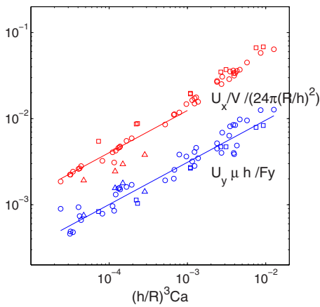
FIG. 6. (Color online) Adimensioned velocity components U_x (top) and U_y (bottom), as a function of (h/R)^3 Ca , proportional to the total bubble velocity U . Lines: power fits with Eqs. (2) and (3) are \alpha=0.51 , a_{\text{wall}}=10.9 , and a_{\text{fluid}}=4.0 . Only the values U_x/V < 0.5 are fitted. Same symbols than in Fig. 4.
