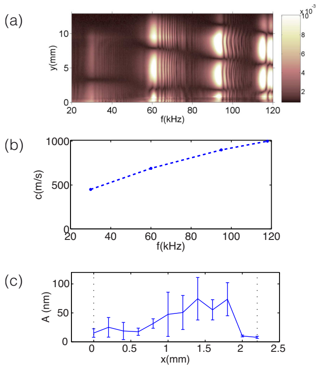
FIG. 2. (Color online) Vibration of the free glass rod, before molding in PDMS: (a) spatial-frequency diagram of the resonating rod. y=0 corresponds to the free end, the forced end (the piezoelectric) is approximately at y=25 mm. The color bar indicates the zero to peak voltage values measured on the hydrophone. (b) Wave speed obtained with the spatial Fourier transform, same scale of the abscisses as in (a); (c) internal vibration of the top channel wall, after molding and assembly of the circuit, measured just below the glass rod whose limits are shown by dotted lines, along the channel ( x -axis). Each point is an average of the vibration in the width of the channel ( f=62 kHz).
