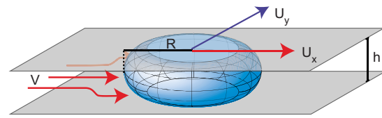
FIG. 3. (Color online) Sketch of the shape of the bubbles confined by the upper and lower faces of the channel.
