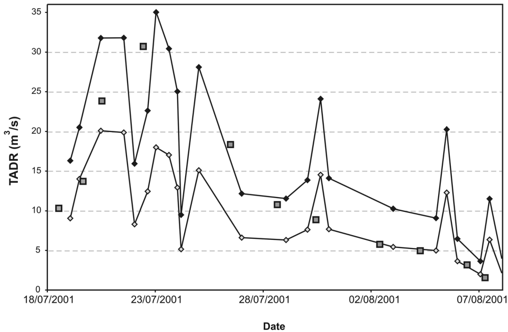
Figure 3. TADR ranges estimated from AVHRR data for lava flow LSF1 active during Etna’s 2001 eruption using the relation given here for Etna in Table 1. Gray squares locate data points obtained by Coltelli et al. [2007] using photogrammetry and DEM subtraction.
