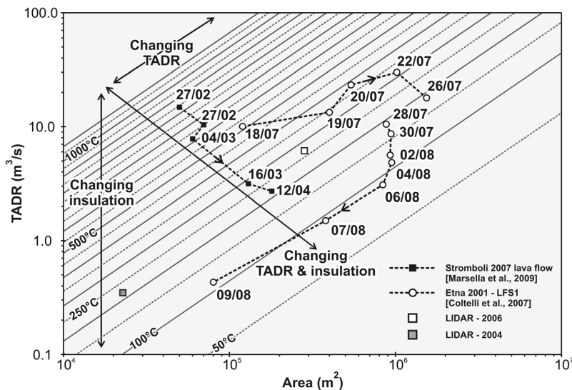
Figure 1. TADR versus lava area relations plotted for Etna using the values of Table 1. Relations are plotted in 50°C increments between T_c of 50°C and 1100°C. Main trends that changes in TADR and/or insulation can cause in the evolution of a lava flow area through time are marked, and available data for Etna and Stromboli are overplotted.
