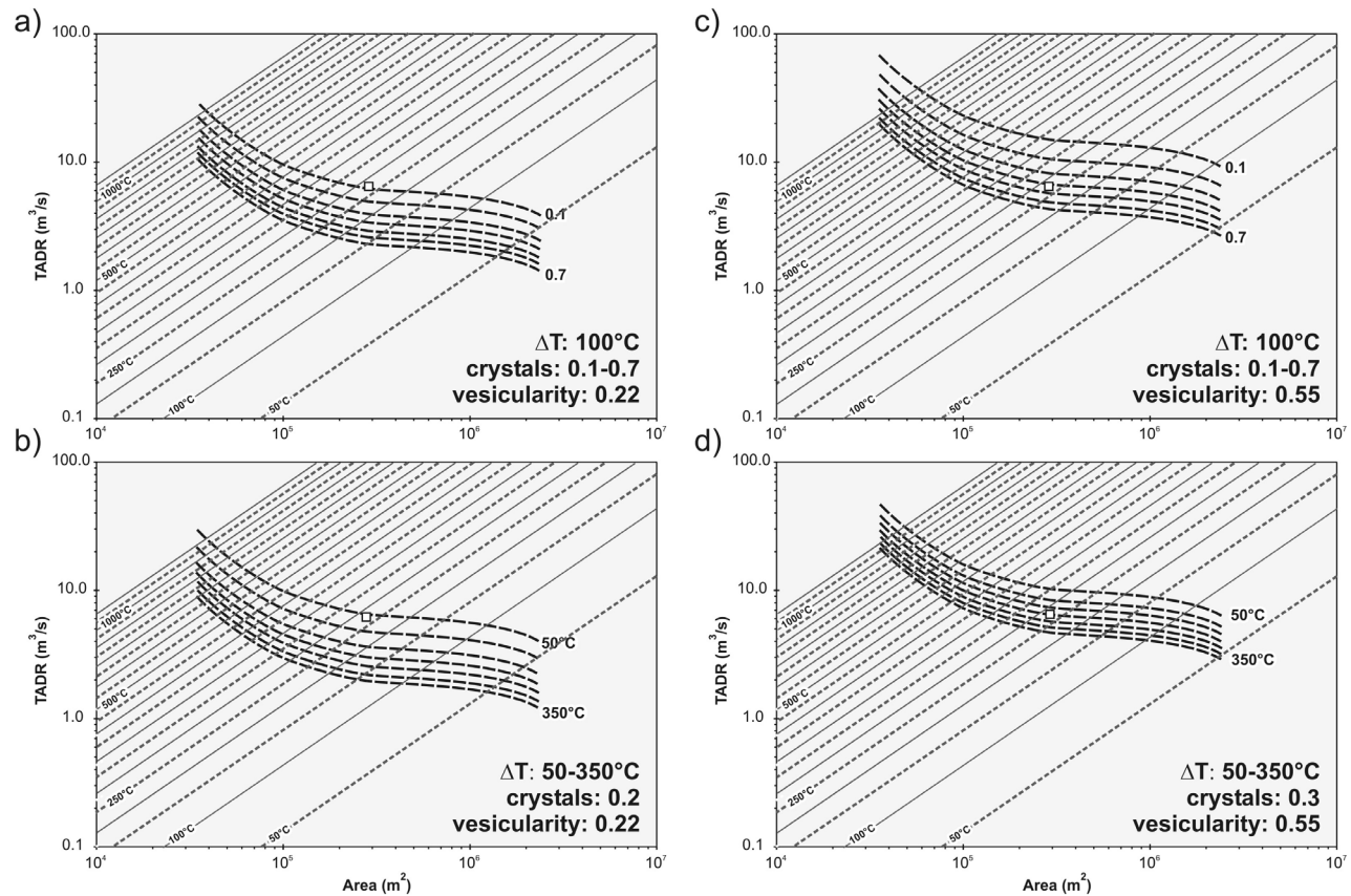
Figure 2. TADR versus lava area relations of Figure 1 with the data point provided by our 17–18 November 2006 lidar data (black square). Each curve represents the solution range for active area and TADR estimates made using an AVHRR image acquired on 17 November 2006 with T_e ranging from 100°C to 1000°C. (a) The solution curves for vesicularity = 0.22, \Delta T = 100^\circ\text{C} and \Delta\varphi in the range 0.1 to 0.7 (in increments of 0.1 between these end points). (b) The solution curves for vesicularity = 0.22, \Delta\varphi = 0.2 and \Delta T in the range 50°C to 350°C (in increments of 50°C between these end points). (c) The solution curves for vesicularity = 0.55, \Delta T = 100^\circ\text{C} and \Delta\varphi in the range 0.1 to 0.7. (d) The solution curves for vesicularity = 0.55, \Delta\varphi = 0.3 and \Delta T in the range 50°C to 350°C.
