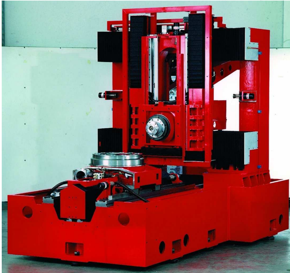
Figure 11. Machining Center structure with preassembled components installed. 386x361mm (72 x 72 DPI)
