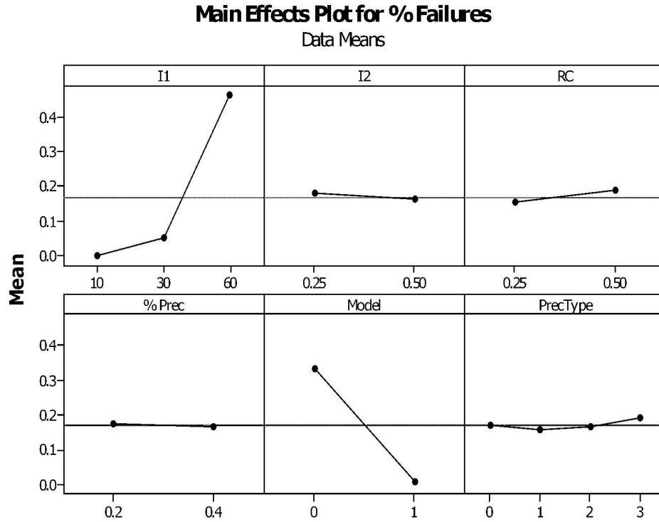
Figure 7. Main Effects Plot for mean failures percentage.
