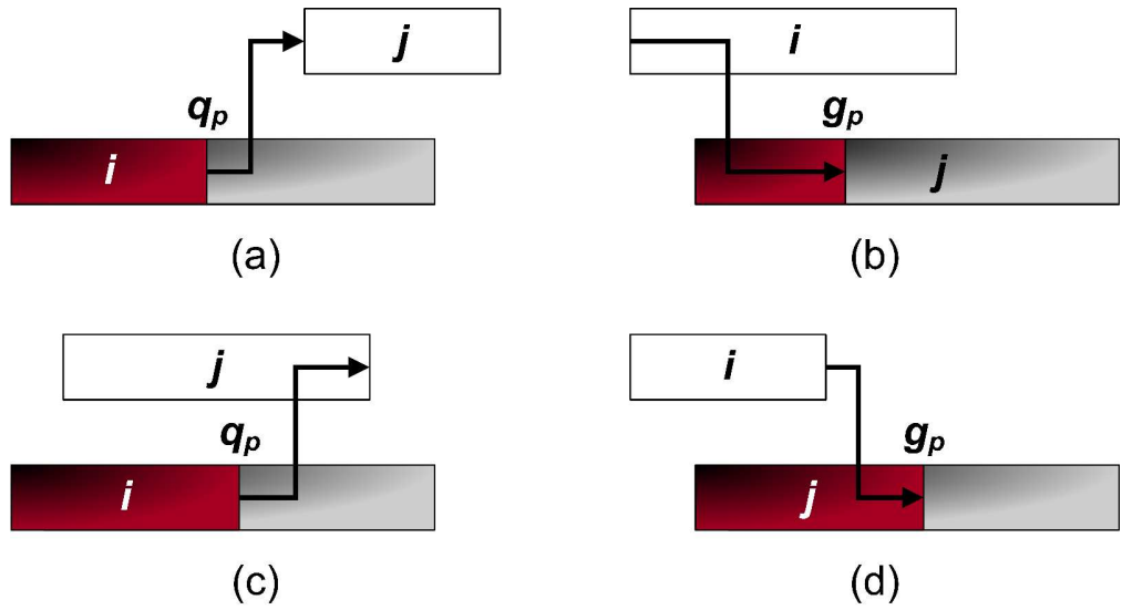
Figure 2. Feeding precedence relations.
