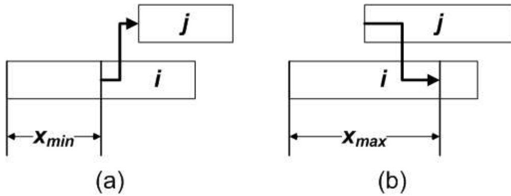
Figure 1. Generalized precedence relations with time lags. 180x68mm (72 x 72 DPI)
