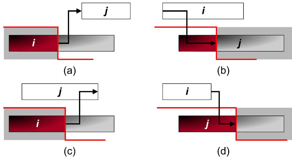
Figure 5. Execution masks for feeding precedence relations.
