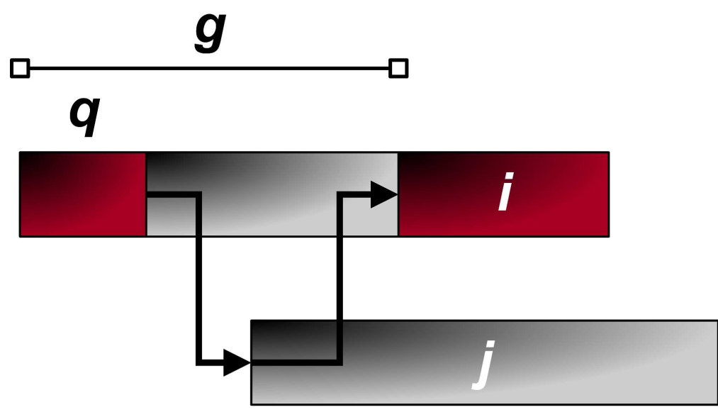
Figure 6. Multiple precedence constraints.
