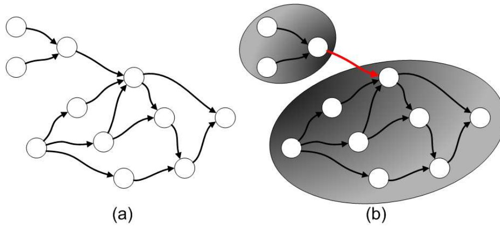
Figure 3. Aggregation of activities. 328x146mm (72 x 72 DPI)
