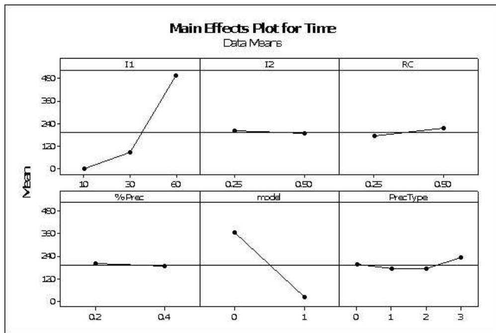
Figure 9. Main Effects Plot for mean solution time.
