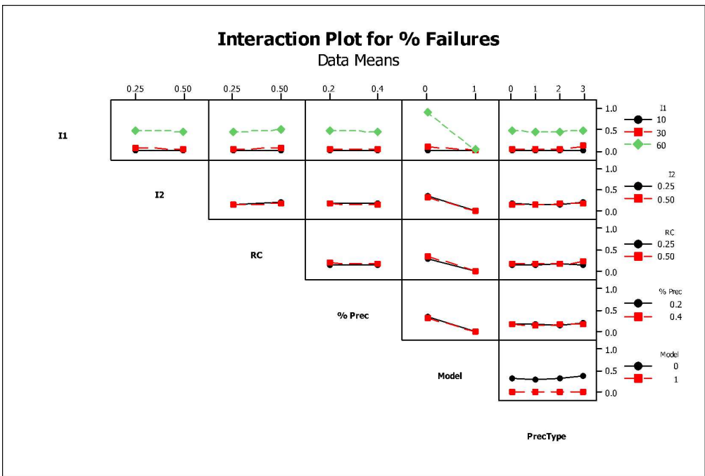
Figure 8. Interaction Plot for mean failures percentage.
