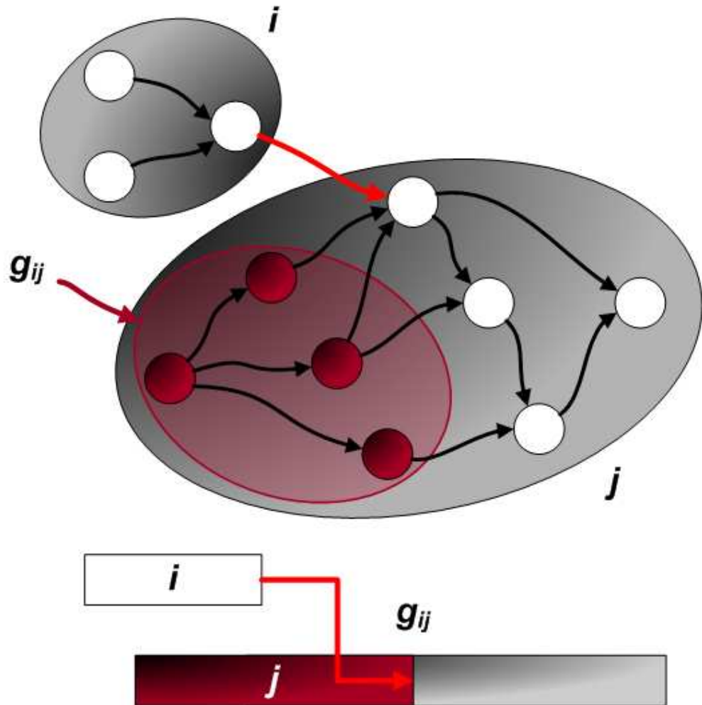
Figure 4. Feeding precedence on aggregate activities. 187x188mm (72 x 72 DPI)
