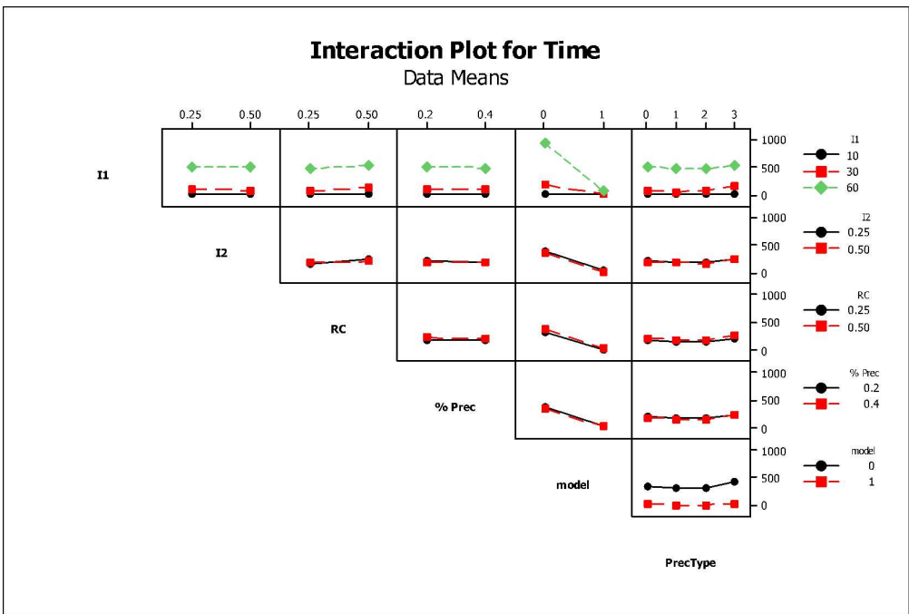
Figure 10. Interaction Plot for mean solution time.
