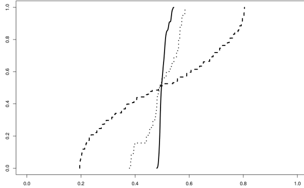
Figure 4: Visual representation of the three conditional distributions considered in the simulation scheme. We plot the empirical cumulative distribution functions of \{g^k(A = 1|W_{(\ell)}) : \ell = 1, \dots, n\} for k = 1 (solid line), k = 2 (dashed line) and k = 3 (dotted line), where W_{(1)}, \dots, W_{(L)} are independent copies of W drawn from the marginal distribution of W under P_0^k (which does not depend on k ), and L = 10^5 .
