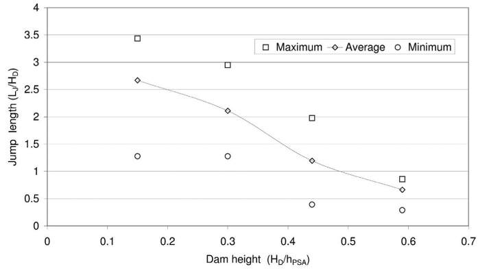
Figure 10.3: Dimensionless jump length of a powder-snow avalanche overflowing a dam. The jump length is given in units of the dam height. (2D Cemagref experiments.)
