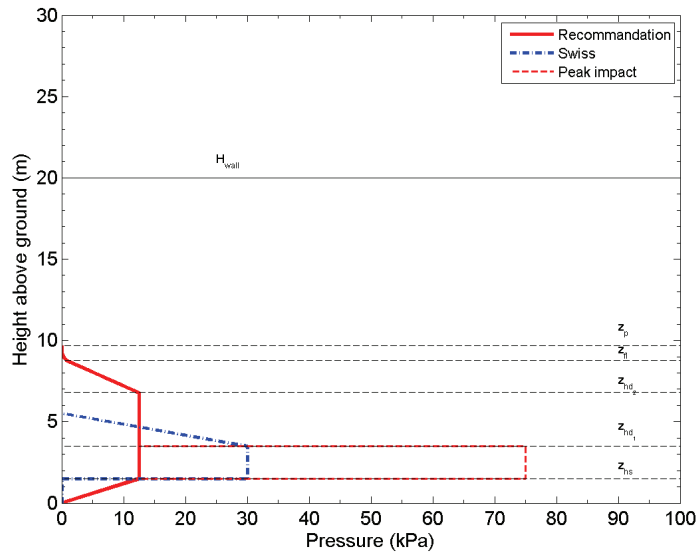
Figure E1: Distribution of impact pressure on a wall for the example, according to the recommendation. An initial impact pressure peak with a magnitude of 3\rho_1 u_1^2 , which may be taken into account in design depending expert judgment, is shown. Also shown is a comparison with Swiss recommendations. Top: example e1; Bottom: example e2.
