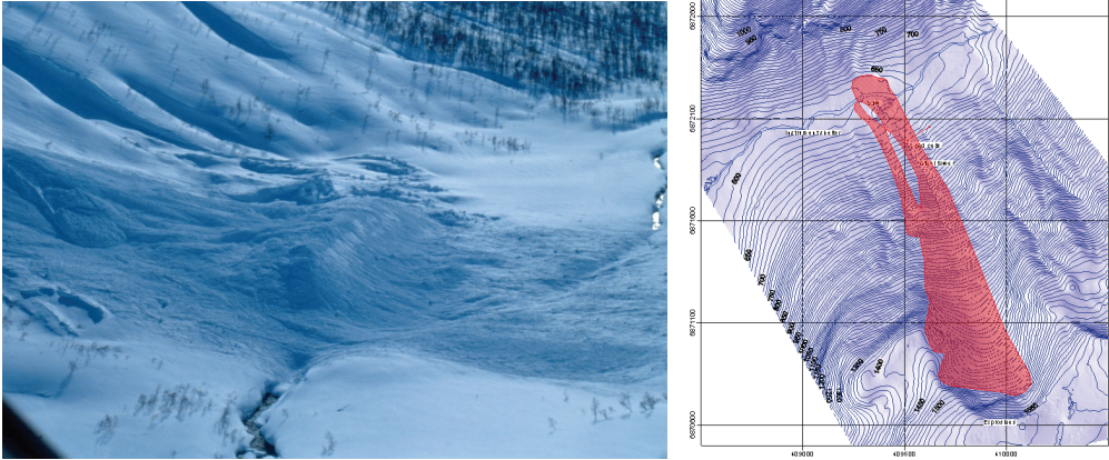
Figure 7.2: Deposition pattern of the 19970208 12:38 avalanche at Ryggfonn. Left : Photograph of the deposit. Right : Map of the deposit. Due to deposits of previous avalanches the effective free board height was only 5 m. The estimated front velocity was 40 \text{ m s}^{-1} . (Photo NGI.)
