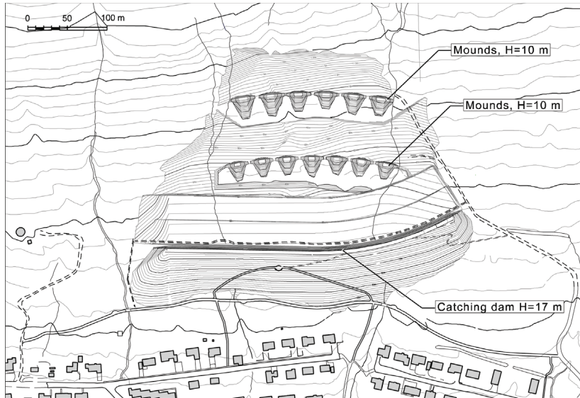
Figure 15.7: Plan view of combined braking mounds and a catching dam, made from reinforced earth. Neskaupstaður, eastern Iceland (designed by VST Consulting Engineers Ltd. and Forverk Consulting Engineers Ltd. in Reykjavík, Iceland, and Cemagref in Grenoble, France).
