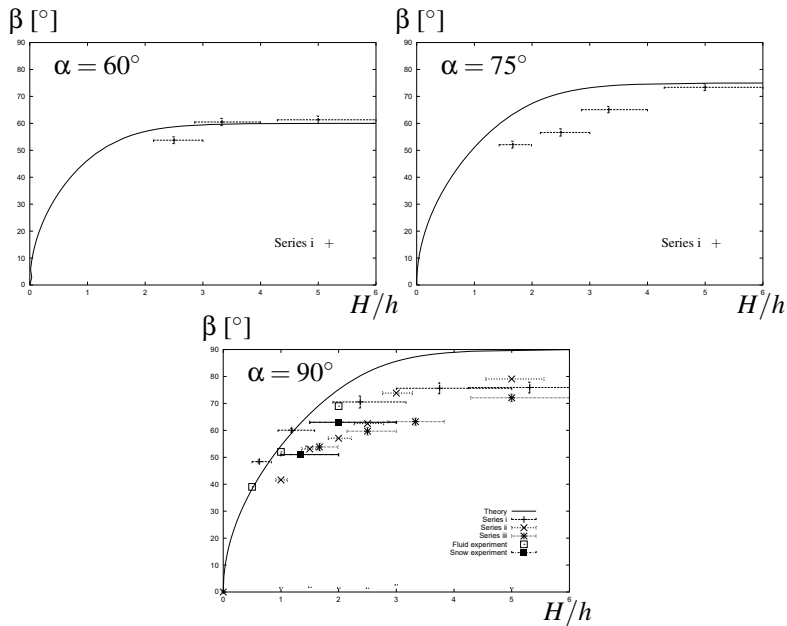
Figure 9.4: The throw angle, \beta , plotted against the non-dimensional mound height, H/h , for different angles between the upstream faces of the mounds and the slope, \alpha . The points denote experimental results and the solid lines are theoretical predictions. ‘Series i, ii and iii’ are results from experiments described in Hákonardóttir and others (2003c) using glass particles on 3, 6 and 9 m long chutes. ‘Snow experiments’ denotes experiments with snow on the 34 m long chute at Weissfluhjoch described in Hákonardóttir and others (2003d), and ‘Fluid experiment’ denotes an experiment described in Yih (1979).
