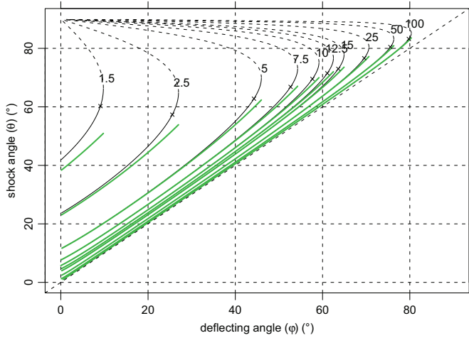
Figure 5.6: Shock angle \theta as a function of deflecting angle, \phi , and Froude number, Fr , for an oblique shock. Thin solid (weak shock) and dashed (strong shock) curves show the shock angle given by the exact oblique shock relations (see Jóhannesson and others, 2008). Thick green curves show the approximate solution defined by Equations (5.10) to (5.12). The curves are labelled with the Froude number and the \times -symbols show the values of the deflecting angle at which the flow downstream of the shock becomes critical.
