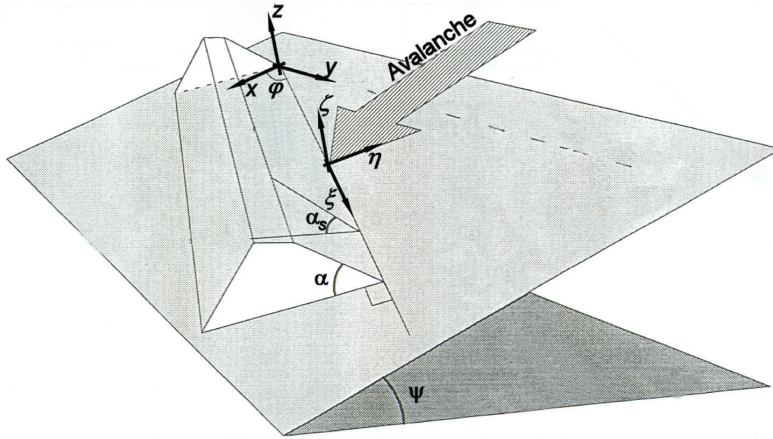
Figure 5.1: A schematic figure of a deflecting dam showing the (x,y,z) - and (\xi,\eta,\zeta) -coordinate systems the deflecting angle, \varphi , the slope of the terrain, \psi , and the angle between the upper dam side and the terrain, \alpha . The figure is adapted from Domaas and Harbitz (1998).
