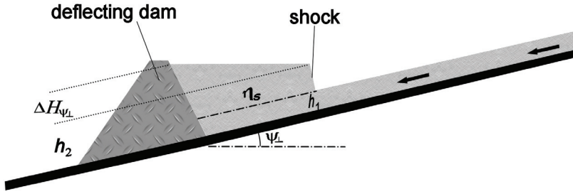
Figure 6.2: A schematic cross section of a shock formed along a deflecting dam built on terrain sloping towards the dam. In a coordinate system moving with the avalanche along the dam, the shock is propagating away from the dam. Material flows across the shock and tends to form a horizontal surface in the direction normal to the dam axis. \psi_{\perp} is the slope of the terrain in the direction normal to the dam axis, and \eta_s is the width of the shock.
