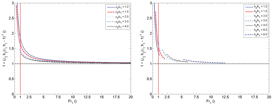
Figure 11.11: Intensity factor f(\text{Fr}_1) = 1 + (\rho_2 h_2 / \rho_1 h_1 - 1)^{-1} versus \text{Fr}_1 . Left : \rho_2 / \rho_1 taken as parameter; h_2 / h_1 \geq 1 . The density ratios between 1 and 4 are chosen to correspond to density ratios in snow avalanches. Right : h_2 / h_1 taken as parameter; densification \rho_2 / \rho_1 ranges between 1 and 5.
