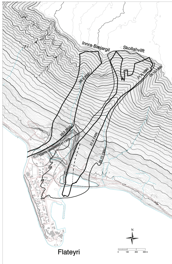
Figure 6.5: Outlines of avalanches that were deflected by the deflecting dams at Flateyri, northwestern Iceland, in 1999 and 2000. The outline of the catastrophic avalanche in 1995 is also shown. The channelised flow of the 1999 avalanche from Skollahvilft along the deflecting dam is indicated by a dashed curve. Hypothetical outlines of the avalanches in 1999 and 2000 in the absence of the deflecting dams are shown as dotted curves. Due to the channelised flow along the dam, the run-out of the 1999 avalanche may have been increased by a distance on the order of 100 m.
