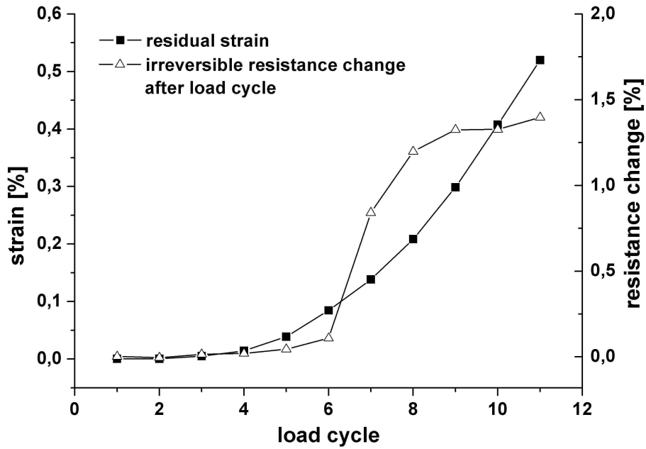
Figure 6: Apparent residual strain at the end of each loading cycle and corresponding irreversible resistance change, measured during the cyclic tensile test.
