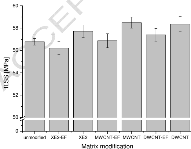
Figure 2: Interlaminar shear stresses of the modified GF-NCF-EP materials (EF = electrical field applied during curing).
