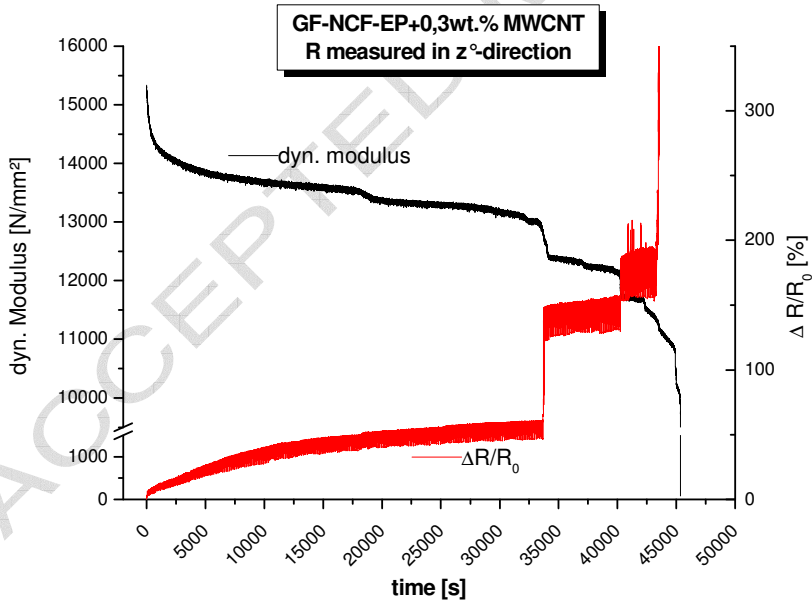
Figure 9: Stiffness and resistance change for a specimen under dynamic tensile load. Resistance measured in thickness (Z)-direction.
