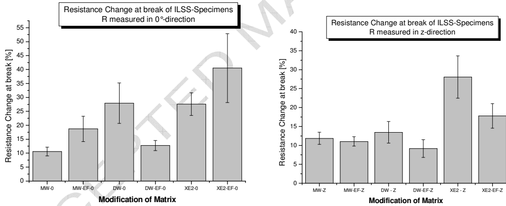
Figure 4: Resistance change at break of all tested materials; a) measured in length direction of the specimens, b) measured in thickness direction of the specimens (EF = electrical field applied during curing).
