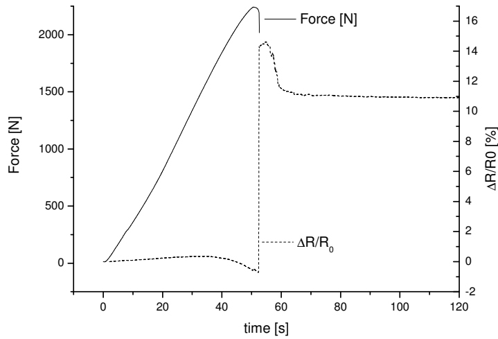
Figure 3: Progression of force and resistance change during ILSS test.
