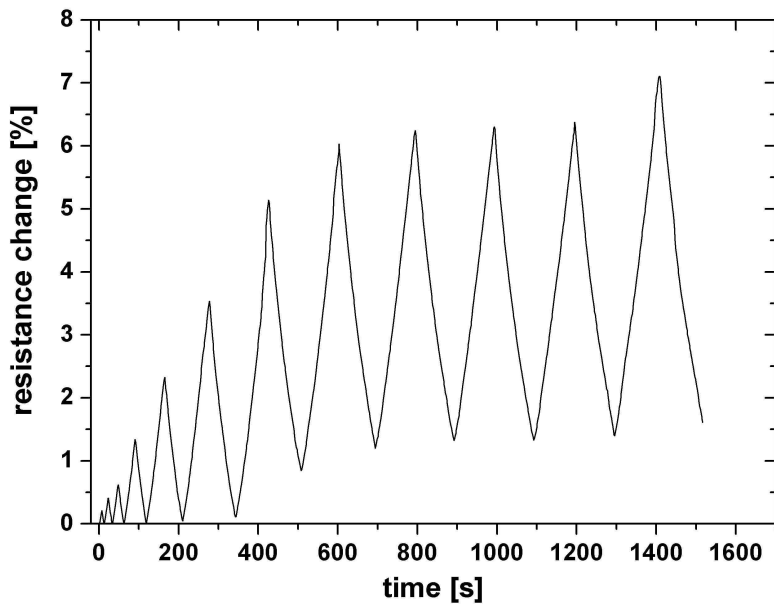
Figure 5.: a) Measured stress and strain and b) electrical resistance change during a stepped tensile test. The specimen contained 0.3 wt.% MWCNTs in the matrix and the resistivity was measured in z-direction.
