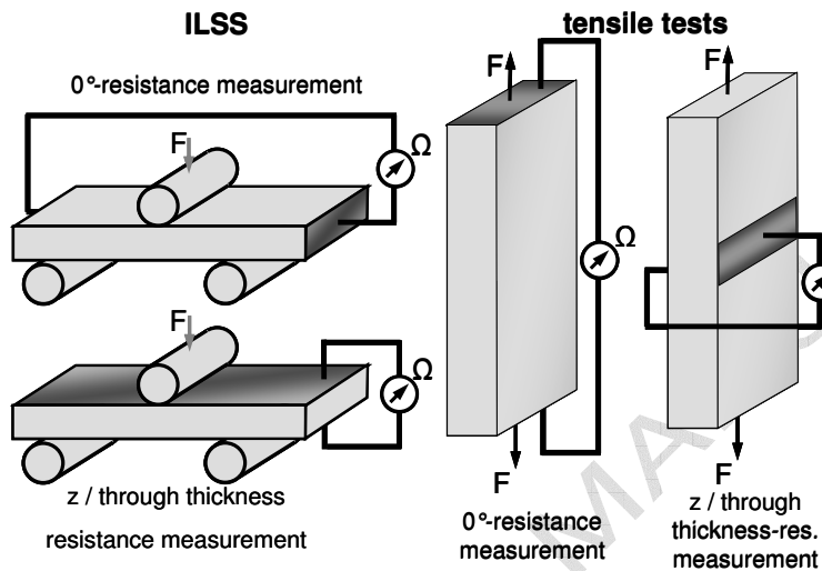
Figure 1: schematic visualization of specimen for in-situ resistance measurements during ILSS test (left) and tensile-test (right).
