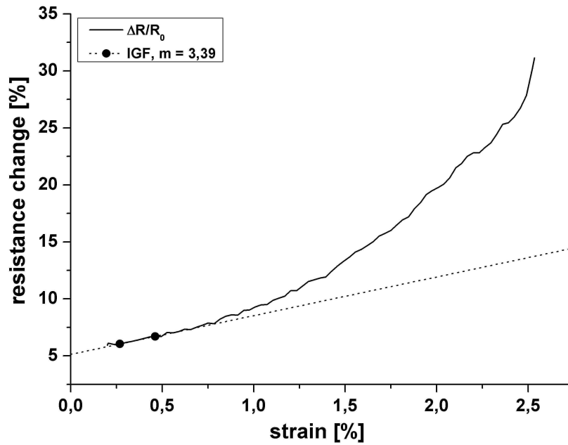
Figure 7: Electrical resistance change vs. mechanical strain, measured during the 10 th loading cycle of a cyclic tensile test (resistivity measured in z-direction) for a) the composite containing 0.3 wt.% of MWCNTs and b) the composite containing 0.3 wt.% of carbon black.
