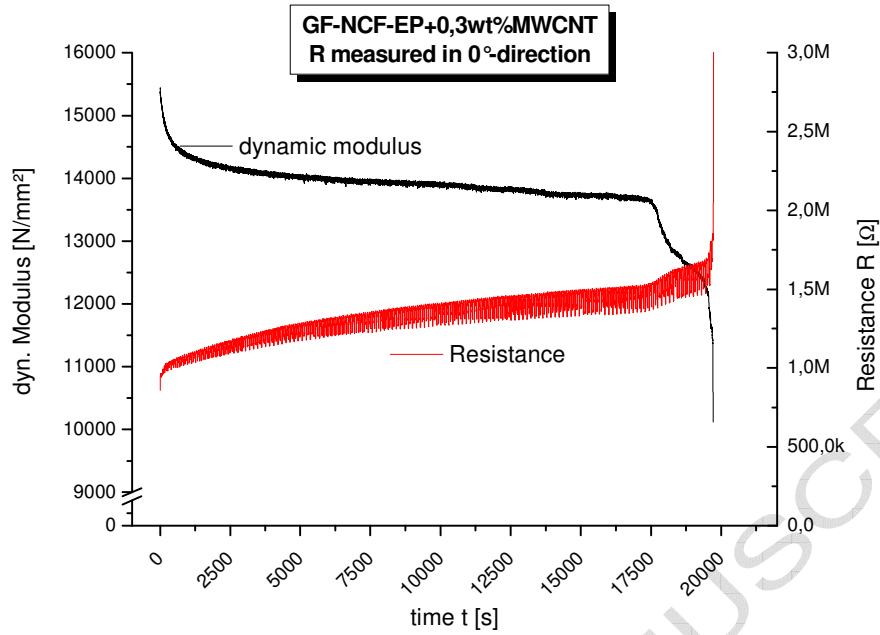
Figure 8: Stiffness and resistance change for a specimen under dynamic tensile load. Resistance measured in longitudinal (0°)-direction.
