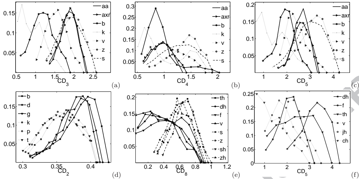
Fig. 2. Density of selected single feature vector elements related to correlation dimension, indicative of phonemes from different classes: vowels, fricatives and stops. Top row: feature vector elements for selected phonemes from mixed classes are (a) CD_3 = \mu(D_C) , (b) CD_4 = \sigma(D_C) , (c) CD_5 = \mu(D_C(r_{min}, \bar{r})) . Bottom row: cases of stops, affricatives and fricatives for (d) CD_2 = \sigma(C) , (e) D_8 = \sigma(D_C(\bar{r}, r_{max})) , (f) CD_5 feature vector elements.
