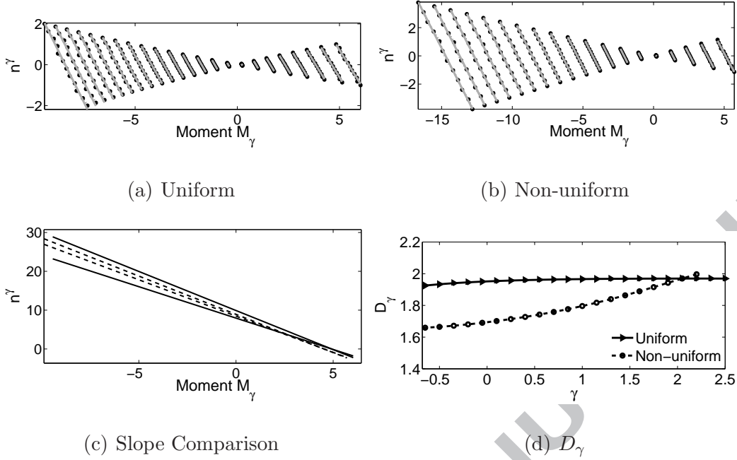
Fig. 3. Construction of the D_\gamma curve: slopes of the n^\gamma versus M_\gamma data points superimposed with the corresponding mean slope fits for the (a) uniform and (b) non-uniform Sinai system; (c) explicit schematic comparison of the minimum and maximum slopes of (a) and (b) for the case of uniform (dashed line) versus the non-uniform case (solid line). (d) The resulting D_\gamma curves.
