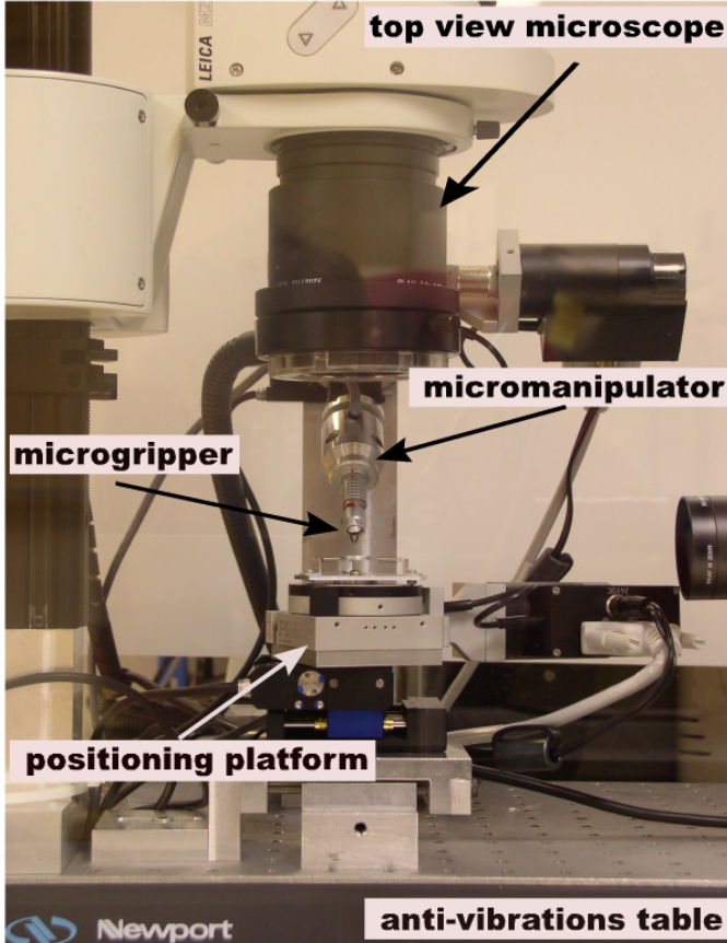
Fig. 2. Photography of the micromanipulation workcell.
