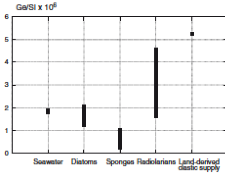
Fig. 5. Values of the Ge/Si ratio of the mean terrigenous supply, seawater and main opalsecreting organisms.
