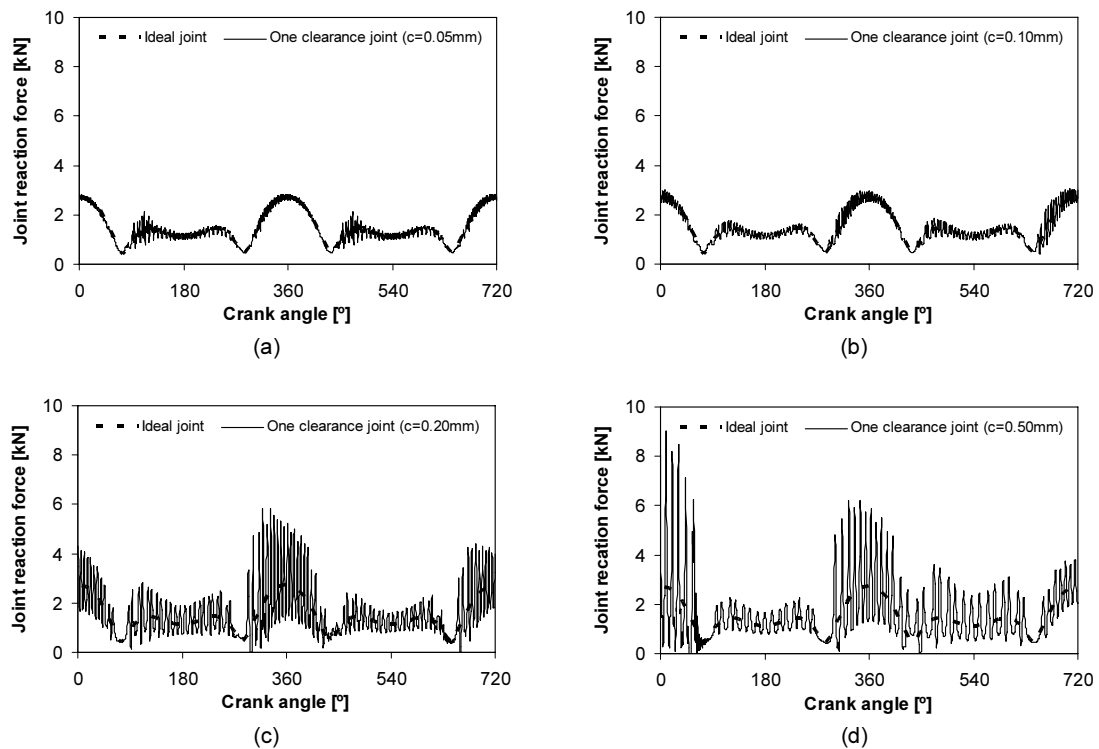
Figure 7. Joint reaction force for different diametric clearance sizes: (a) c=0.05 mm; (b) c=0.10 mm; (c) c=0.20 mm; (d) c=0.50 mm.
