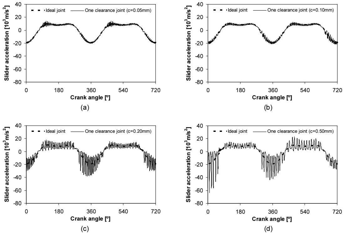
Figure 6. Slider acceleration for different diametric clearance sizes: (a) c=0.05 mm; (b) c=0.10 mm; (c) c=0.20 mm; (d) c=0.50 mm.
