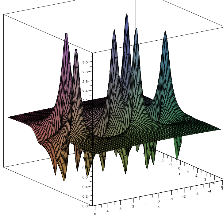
Figure 5: Solution to the NLS equation for N=3 with d_1 = 1 , d_2 = 2 , d_3 = 3 , \tilde{a}_1 = 10000 , \tilde{a}_2 = \tilde{a}_3 = 0 , \tilde{b}_1 = 10000 , \tilde{b}_2 = \tilde{b}_3 = 0 .
