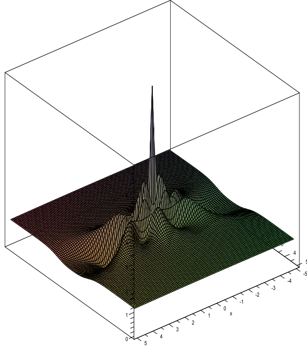
Figure 4: Solution to the NLS equation for N=3 with d_1 = 1, d_2 = 2, d_3 = 3, \tilde{a}_1 = \tilde{a}_2 = \tilde{a}_3 = \tilde{b}_1 = \tilde{b}_2 = \tilde{b}_3 = 1 .
