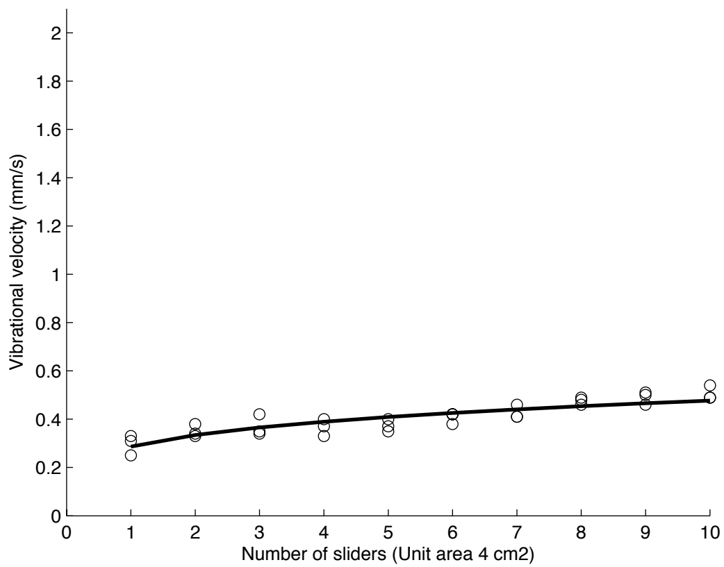
Figure 5: Experiment 1: RMS-vibrational velocity versus number of sliders. Plate 200x300x2mm, high damping ( T_r=0.4s ), thick sliders 20x20x20mm, low roughness R_a=1\mu m . \circ , measurement; - , linear regression in log-log plot.
