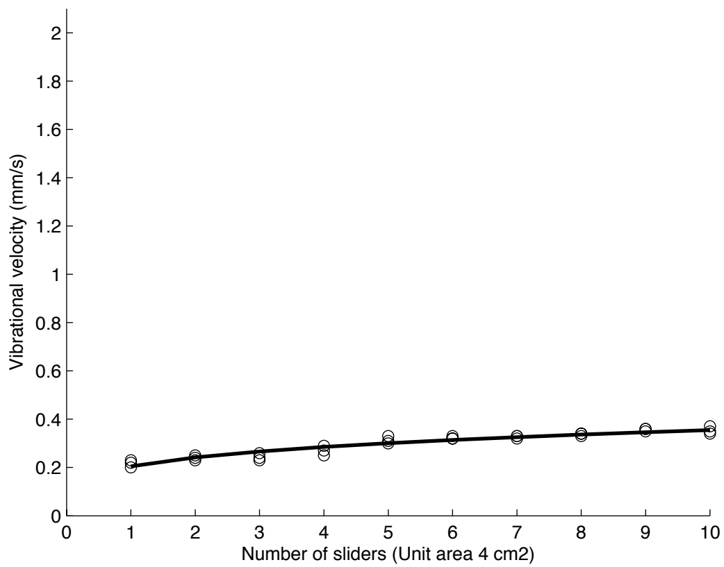
Figure 9: Experiment 3: RMS-vibrational velocity versus number of sliders. Plate 200x300x2mm, high damping ( T_r=0.4s ), thin sliders 20x20x10mm, low roughness R_a=1\mu m . \circ , measurement; - , linear regression in log-log plot.
