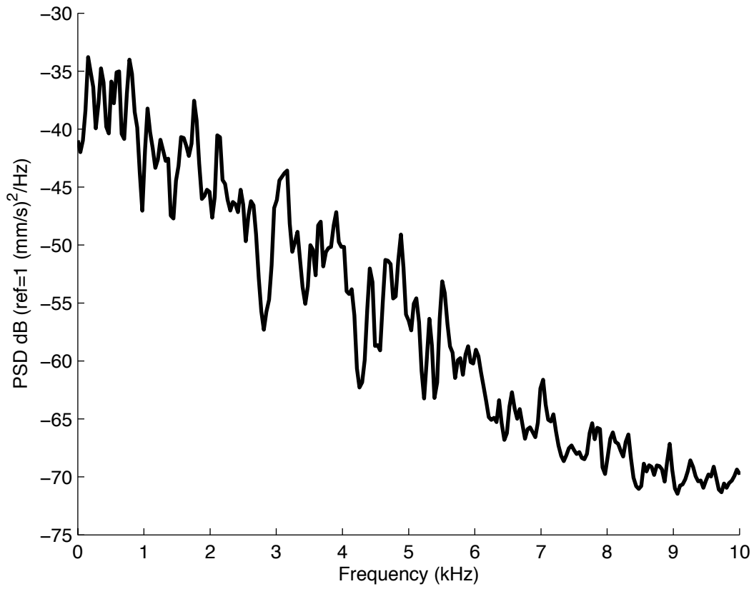
Figure 3: Example of roughness noise. Power spectrum density: Hanning window - 1024 lines - resolution 39 Hz - 127 averages - overlap 20 %.
