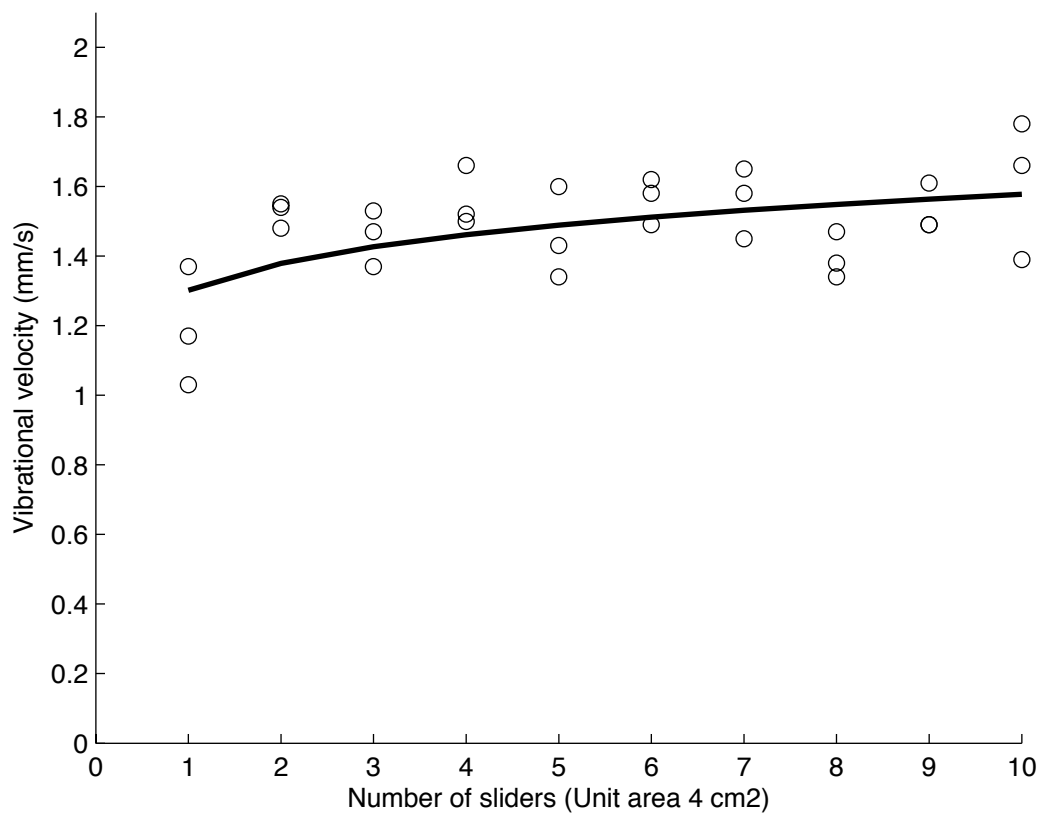
Figure 7: Experiment 2: RMS-vibrational velocity versus number of sliders. Plate 200x300x2mm, low damping ( T_r=21s ), thick sliders 20x20x20mm, low roughness R_a=1\mu m . \circ , measurement; - , linear regression in log-log plot.
