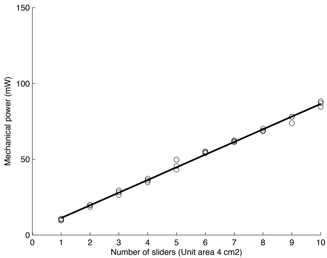
Figure 6: Experiment 2: Mechanical power versus number of sliders. Plate 200x300x2mm, low damping ( T_r=21s ), thick sliders 20x20x20mm, low roughness R_a=1\mu m . \circ , measurement; - , linear regression.
