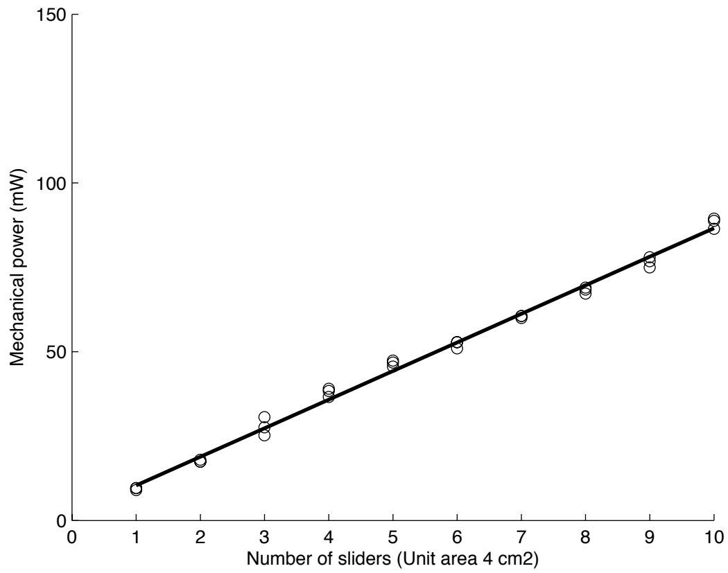
Figure 4: Experiment 1: Mechanical power versus number of sliders. Plate 200x300x2mm, high damping ( T_r=0.4s ), thick sliders 20x20x20mm, low roughness R_a=1\mu m . \circ , measurement; - , linear regression.
