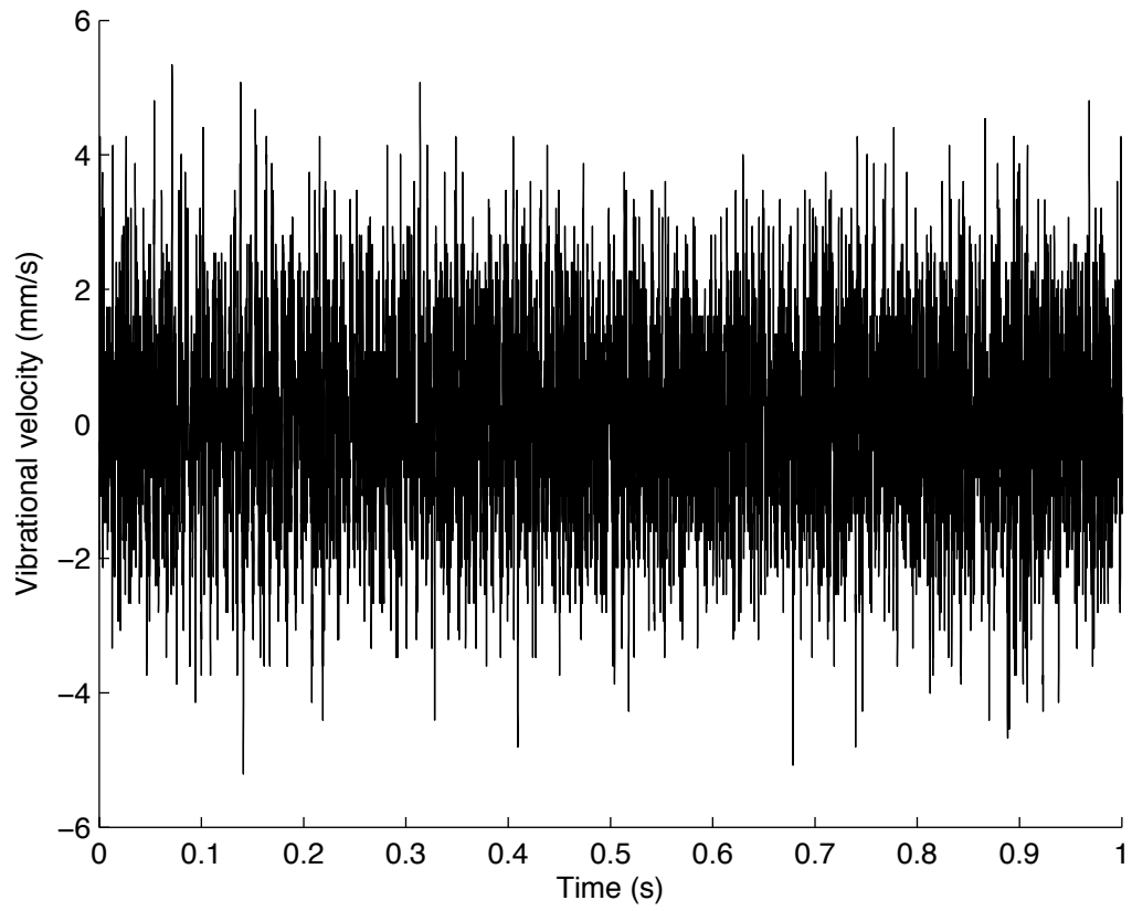
Figure 2: Example of roughness noise. Vibrational velocity versus time measured by accelerometer.
