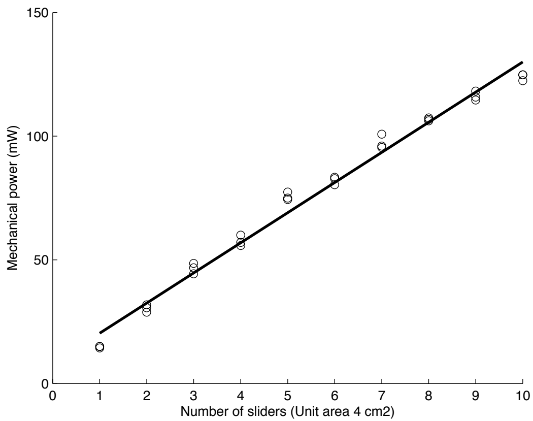
Figure 10: Experiment 4: Mechanical power versus number of sliders. Plate 200x300x2mm, high damping ( T_r=0.4s ), thick sliders 20x20x20mm, high roughness R_a=5\mu m . \circ , measurement; - , linear regression.
