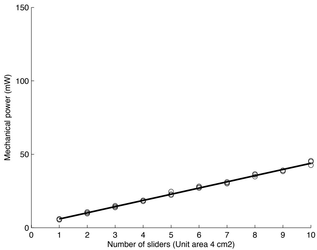
Figure 8: Experiment 3: Mechanical power versus number of sliders. Plate 200x300x2mm, high damping ( T_r=0.4s ), thin sliders 20x20x10mm, low roughness R_a=1\mu m . \circ , measurement; - , linear regression.
