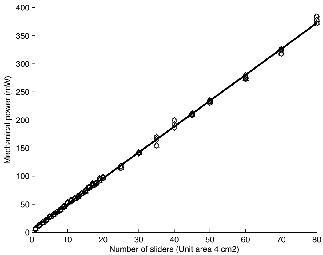
Figure 12: Experiment 5: Mechanical power versus number of sliders. Plate 300x450x2, sliders 20x20x10mm, roughness R_a=5\mu\text{m} and high damping T_r=0.3\text{s} . \circ , accelerometer 1; \diamond , accelerometer 2; \triangle , accelerometer 3; - , linear regression.
