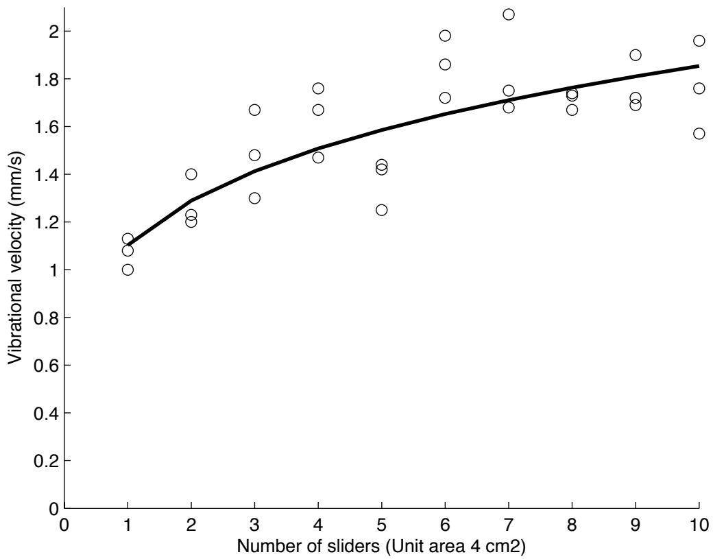
Figure 11: Experiment 4: RMS-vibrational velocity versus number of sliders. Experiment 4: Plate 200x300x2mm, high damping ( T_r=0.4s ), thick sliders 20x20x20mm, high roughness R_a=5\mu m . \circ , measurement; - , linear regression in log-log plot.
