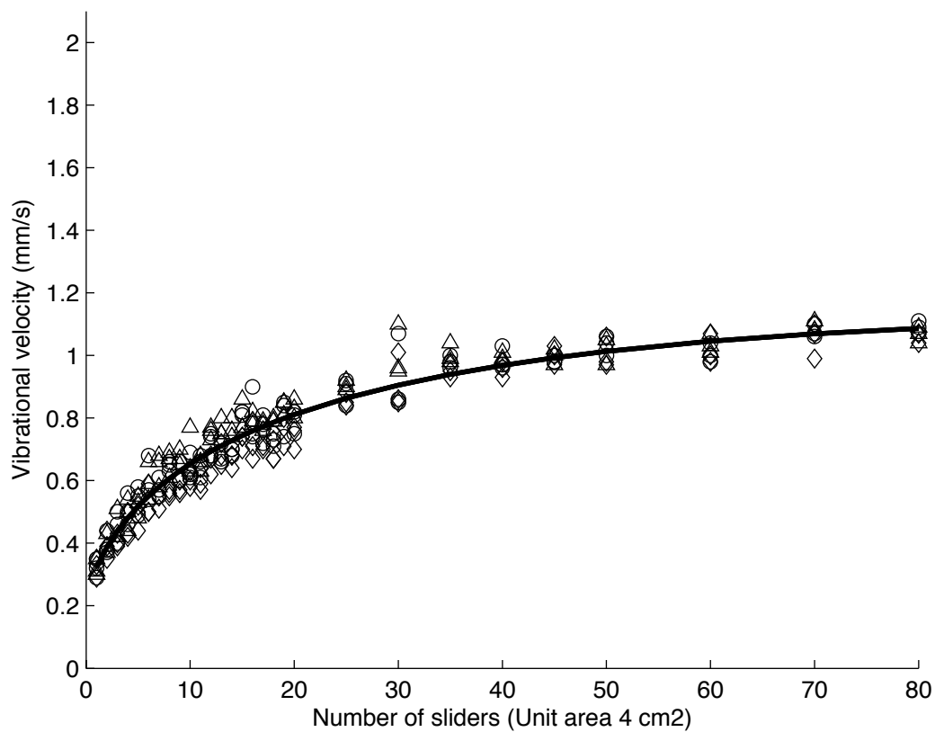
Figure 13: Experiment 5: RMS-vibrational velocity versus number of sliders. Plate 300x450x2, sliders 20x20x10mm, roughness R_a=5\mu\text{m} and high damping \text{Tr}=0.3\text{s} . \circ , accelerometer 1; \diamond , accelerometer 2; \triangle , accelerometer 3; —, polynomial interpolation of degree 3 in log-log plot.
